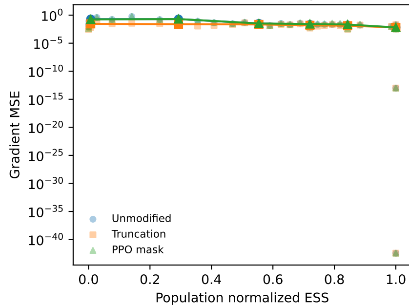
Estimator reliability
