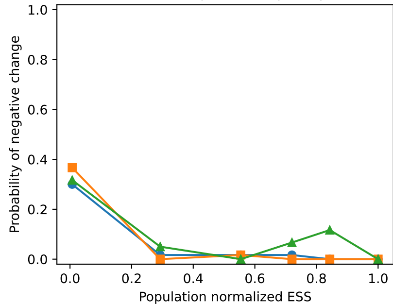
Harmful-update frequency
