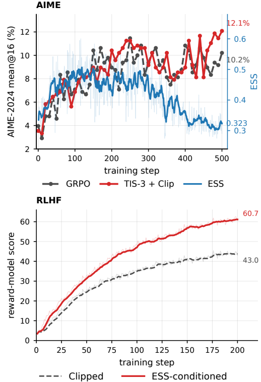
Figure 8: Top: Qwen3-1.7B results over extended training. AIME-2024 result is shown for GRPO (dashed) and TIS-3 + Clip (solid). Blue lined represents ESS for TIS-3 + Clip. Bottom: RLHF on Qwen3-4B-Instruct-2507. End labels report the step-200 observations.
