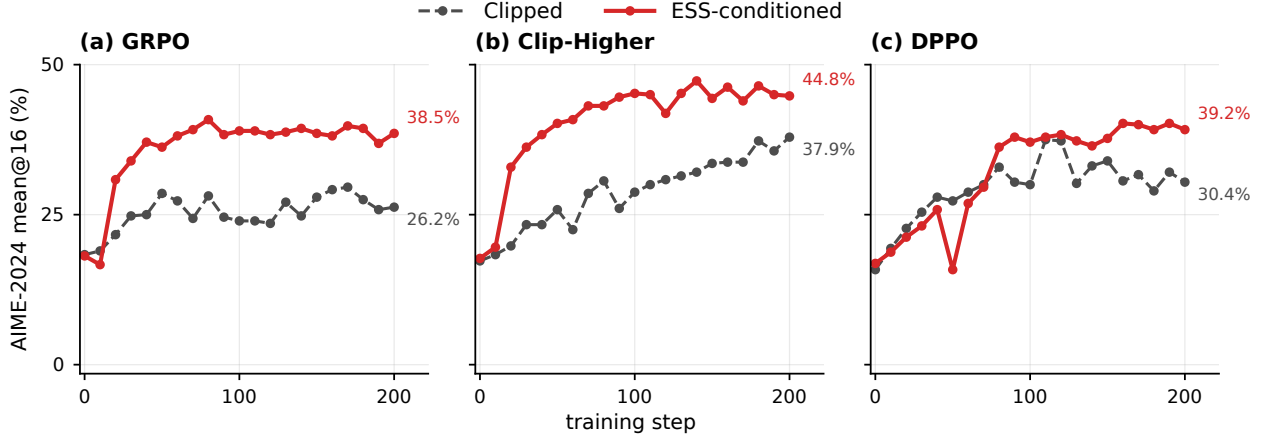
Figure 5: Qwen3-30B-A3B math RLVR results. Dashed curves corresponds to the baseline methods. Solid curves begin with TIS-3 and switch to the corresponding clipped update when ESS falls below 0.1. (a) GRPO clipping. (b) Clip-Higher. (c) DPPO. End labels report the final observed AIME-2024 mean@16.
