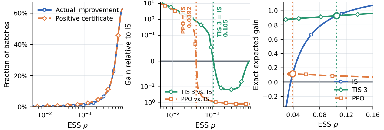
Figure 3: Gaussian-bandit reliability and estimator comparison. From left to right: positive certificates and actual positive improvement under the adaptive IS step; exact expected gain of TIS-3 and PPO relative to IS; and exact expected gain near the pairwise crossovers. Vertical lines and open markers identify the intersections.
