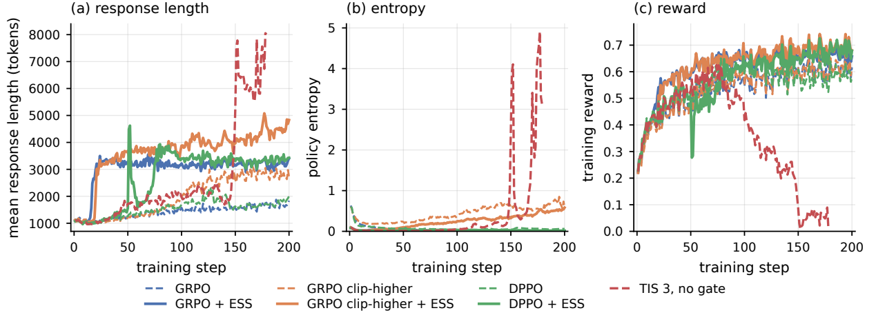
Figure 14: Training dynamics for the main comparisons. The static TIS 3 run develops extreme response length and entropy together with a collapse in training reward. The safeguards and their ESS-conditional variants avoid this failure over the reported 200 steps.
