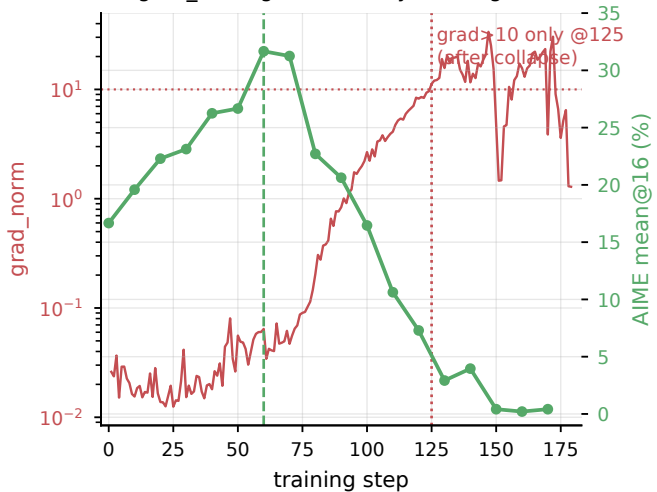
(b) grad_norm gives no early warning
