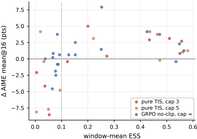
(a) ESS ( r=+0.48 )
