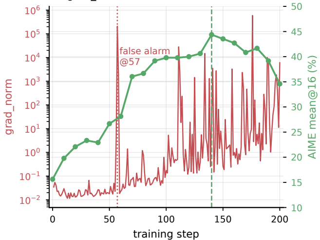
(b) grad_norm coincides
