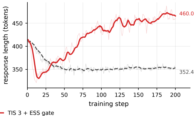
(b) response length
