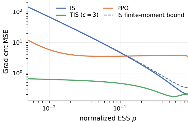
(c) Full-certificate crossover
