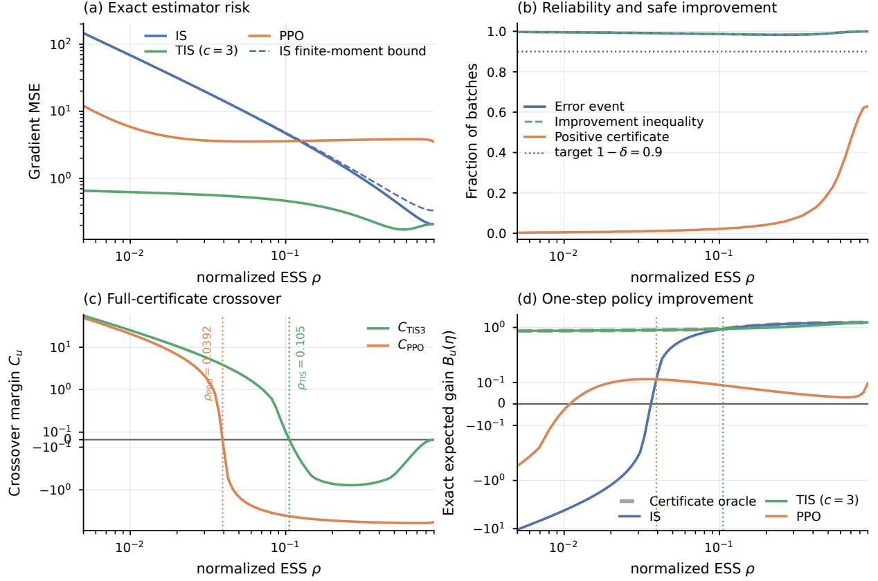
Figure 2: Theory validation in the Gaussian bandit with g = 2 , N = 32 , TIS cap c = 3 , PPO radius \epsilon = 0.2 , and fixed step \eta = 0.4 . (a) Exact estimator MSE and the finite-moment IS MSE envelope in Equation (13). (b) Empirical coverage of the Lemma 2 event and Theorem 3 improvement inequality at confidence 1 - \delta = 0.9 ; the orange curve reports the fraction of batches with a positive certified step. (c) The exact crossover margins in Equation (22); positive values favor the controlled estimator. (d) Exact expected one-step policy improvement at the common fixed step. Vertical lines carry the computed IS–TIS3 and IS–PPO crossovers from (c) into (d).
