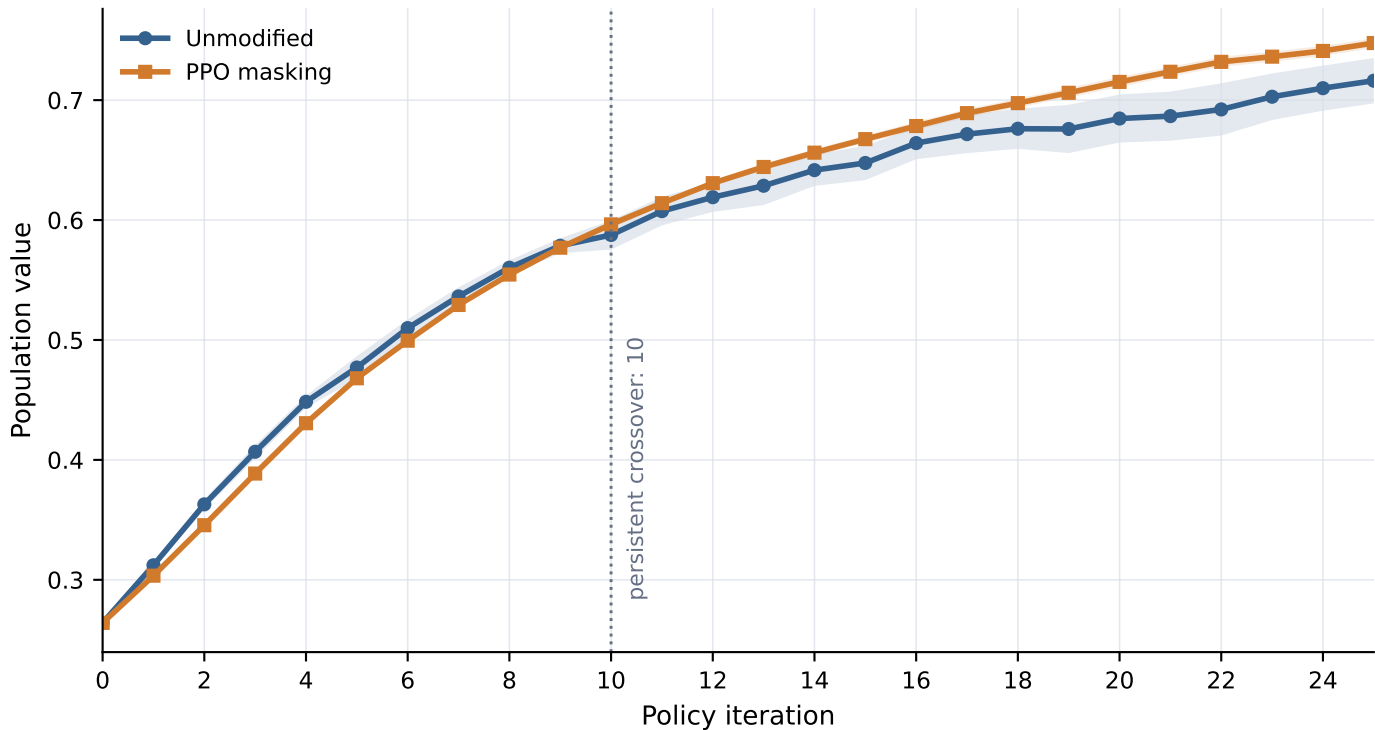
Signal preservation helps early; variance control helps later
