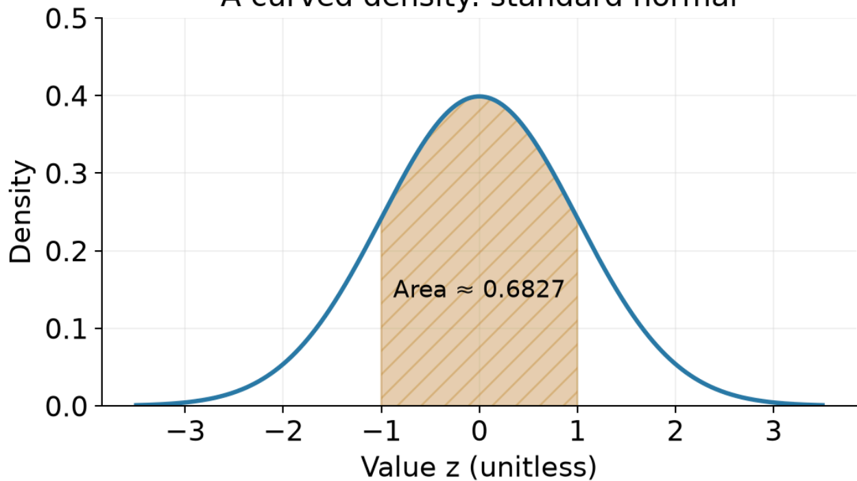
A curved density: standard normal
