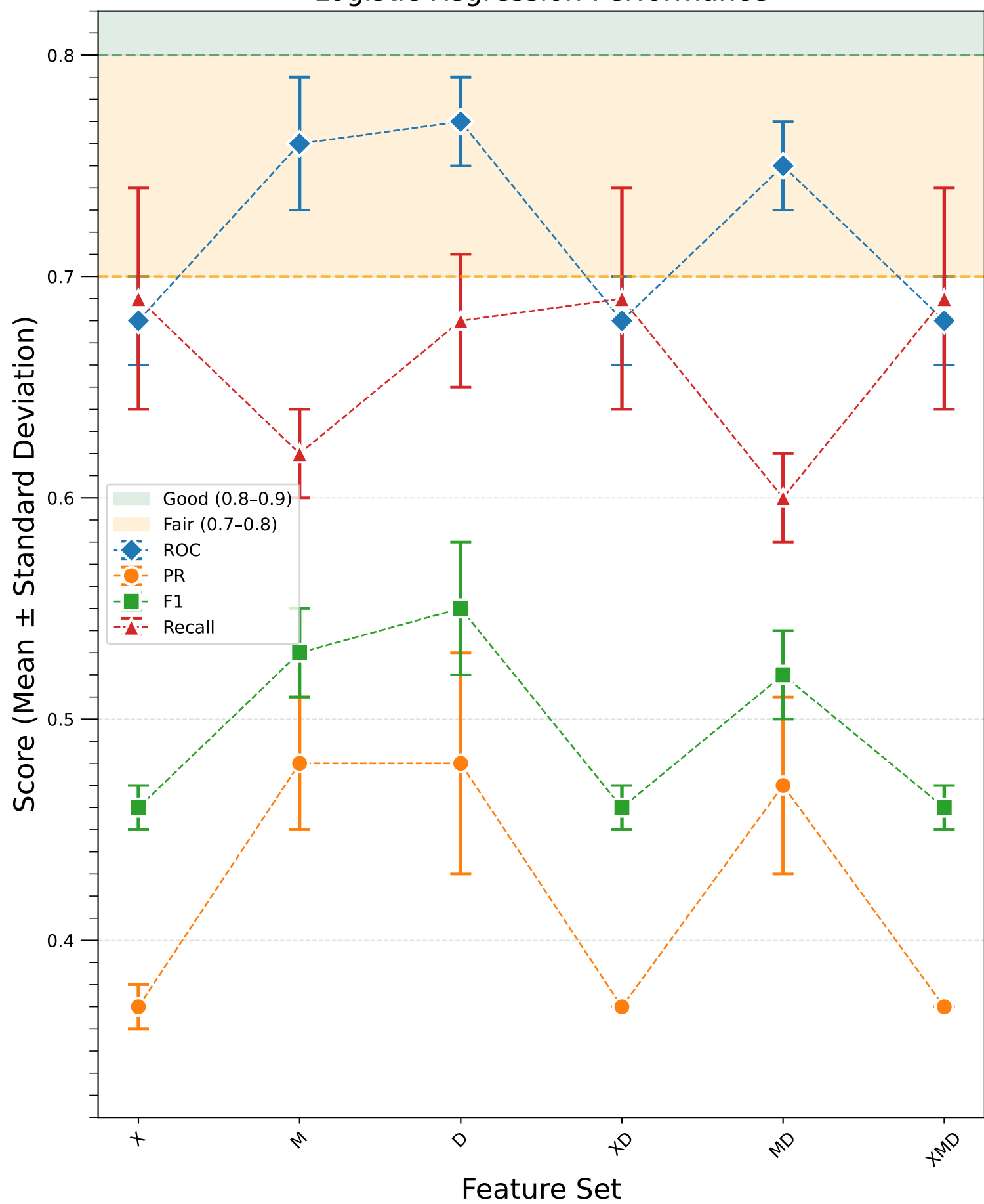
Logistic Regression Performance
