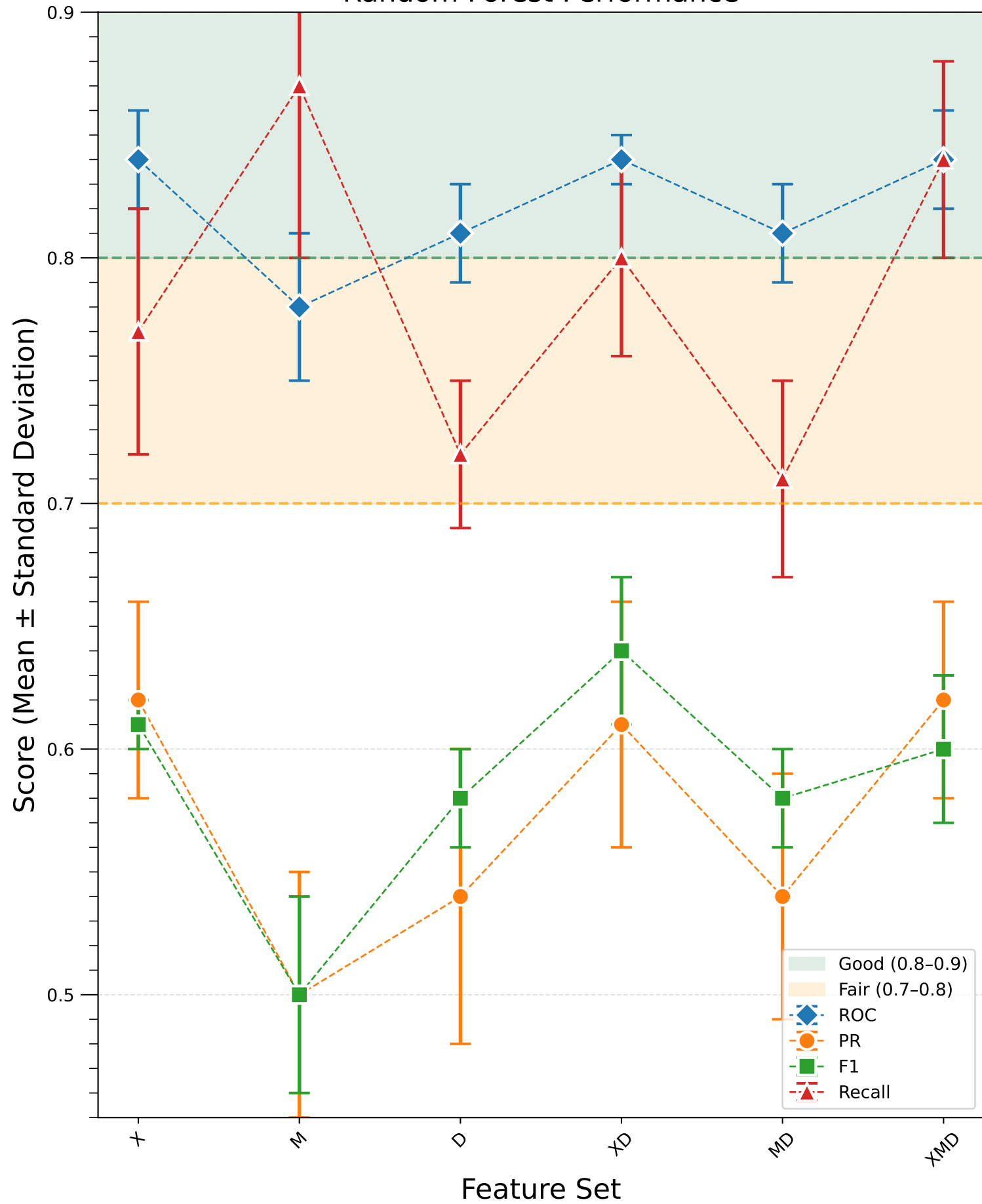
Random Forest Performance
