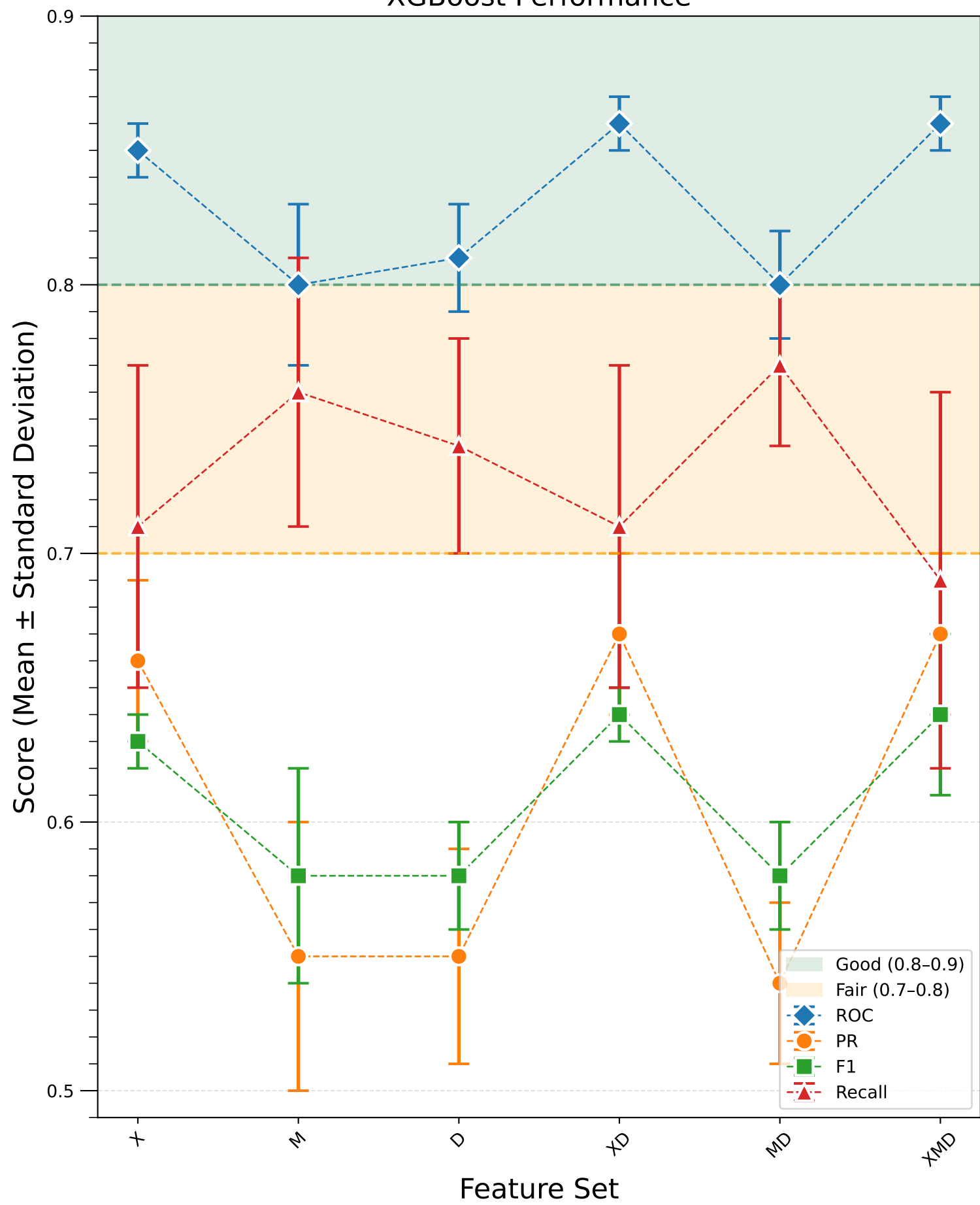
XGBoost Performance
