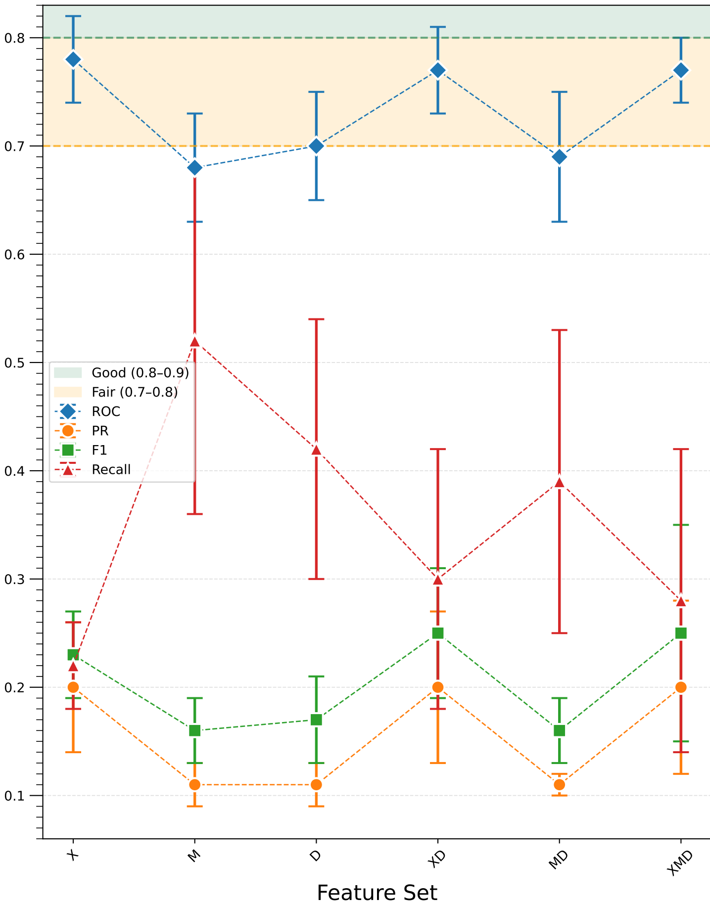
XGBoost Performance
