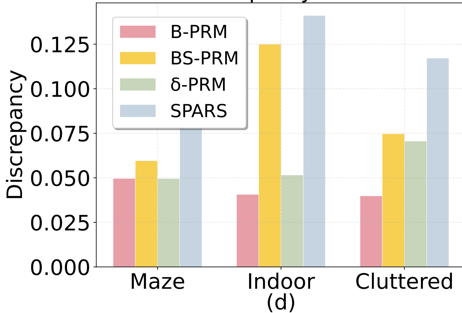
Discrepancy Score
