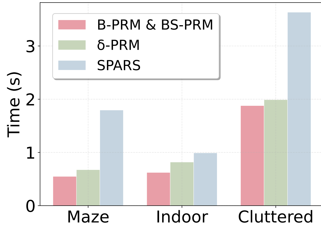
Generation Time
