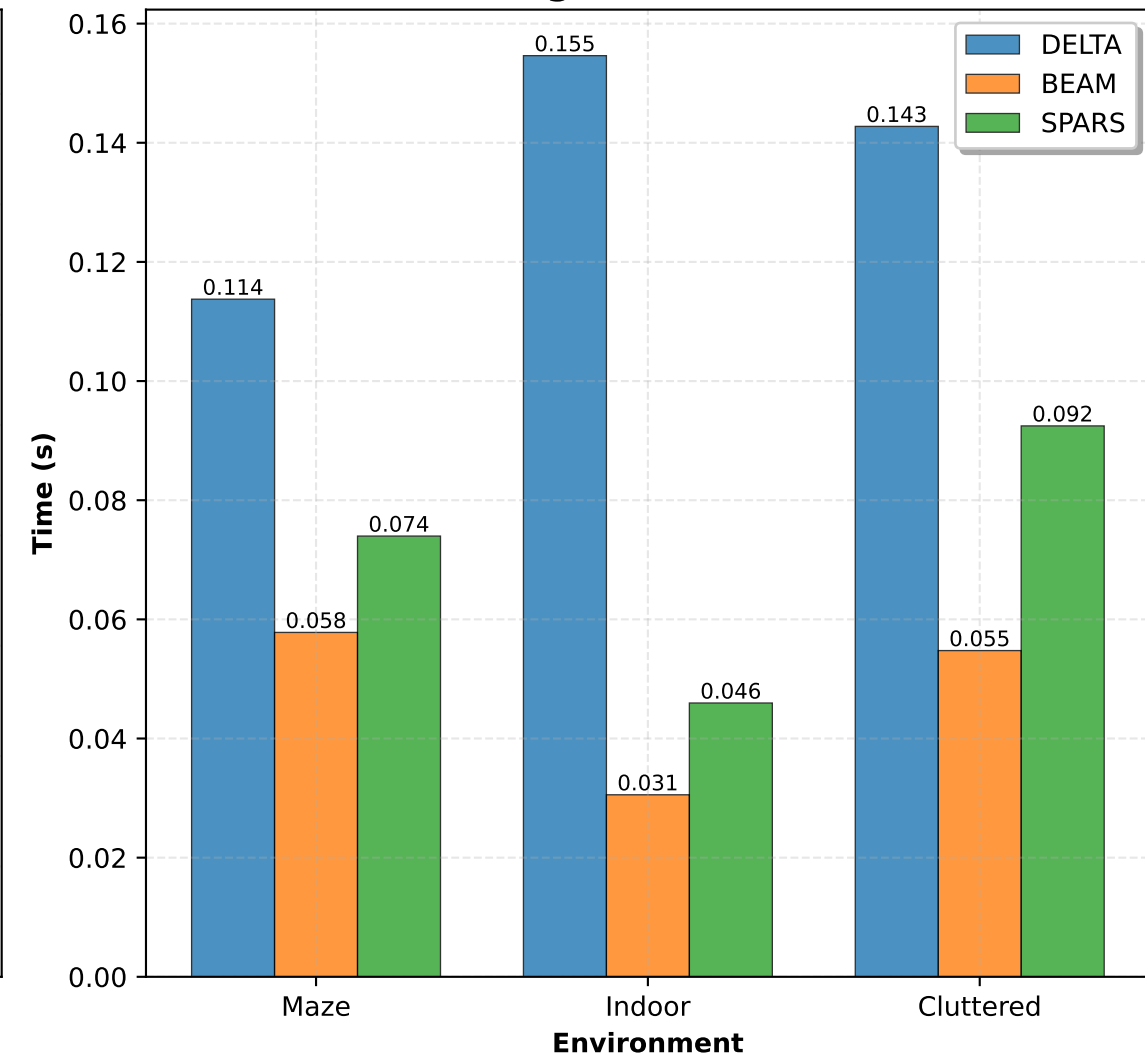
Average Search Time
