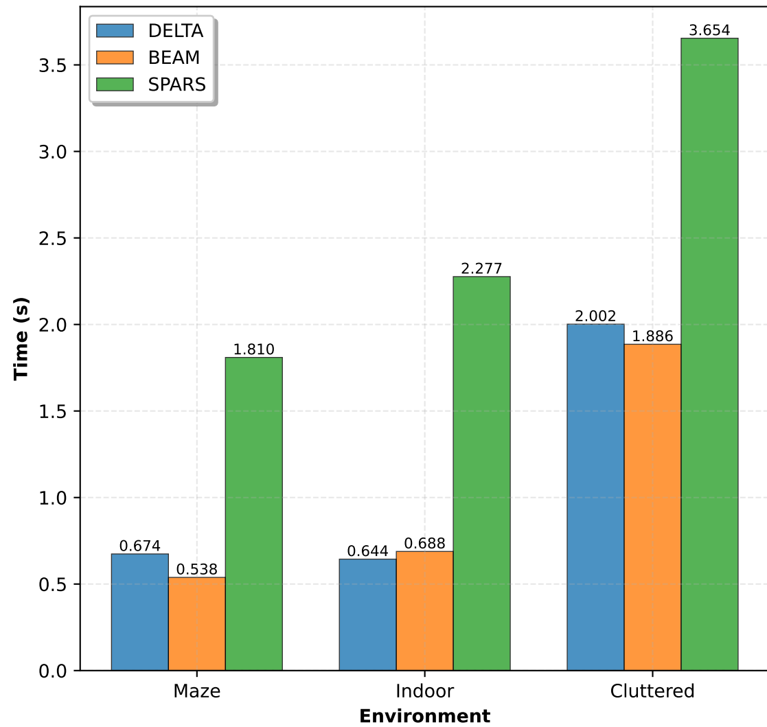
PRM Generation Time
