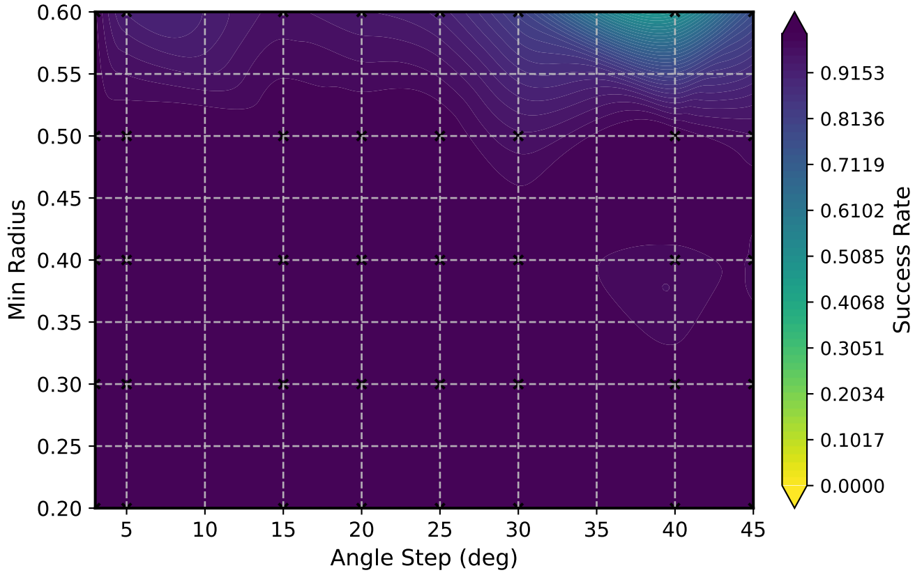
[Indoor] Pathfinding Success Rate
