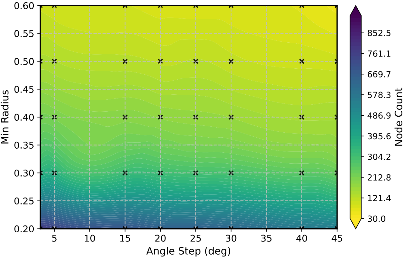
[Maze] Generated Node Density
