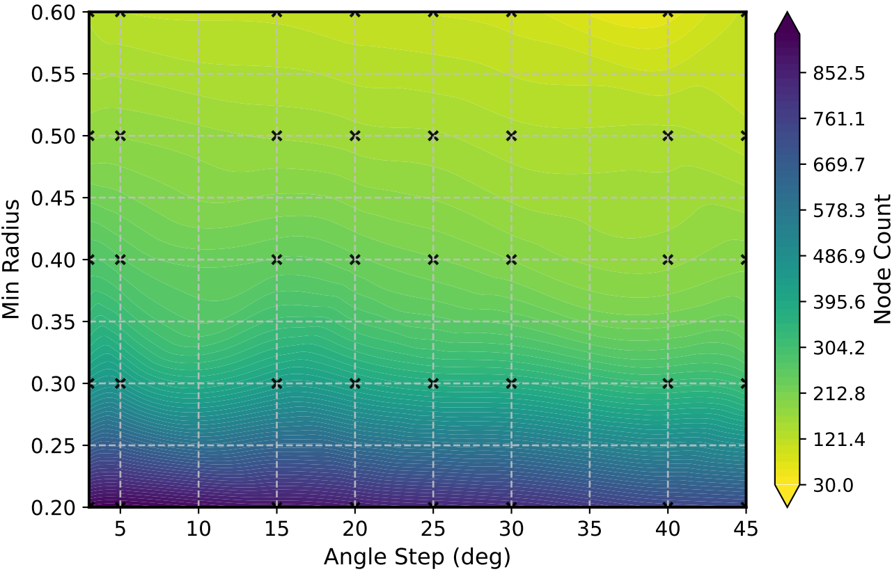
[Indoor] Generated Node Density
