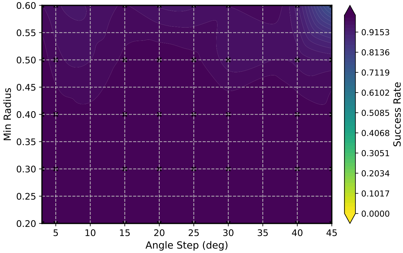
[Maze] Pathfinding Success Rate
