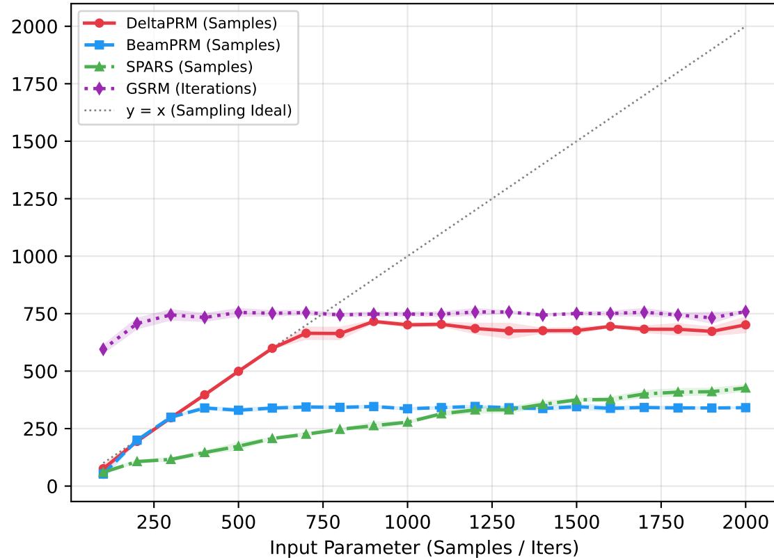
Random Environment (40×40)
