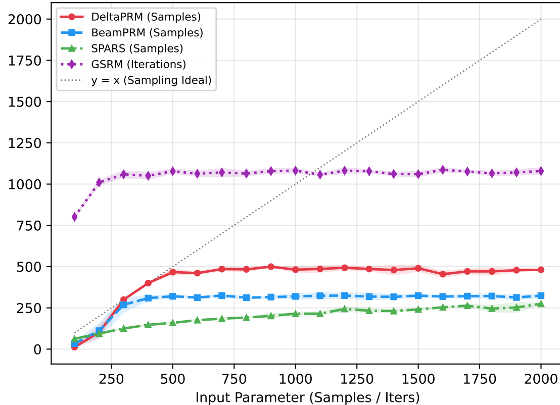
Maze Environment (49×49)
