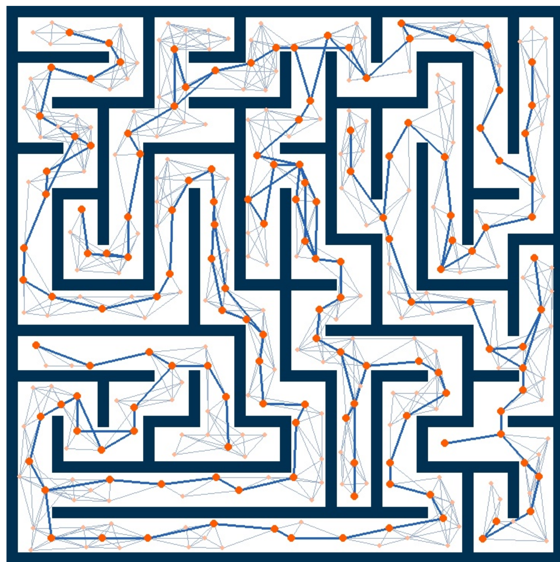
(a2) BS-PRM Maze
