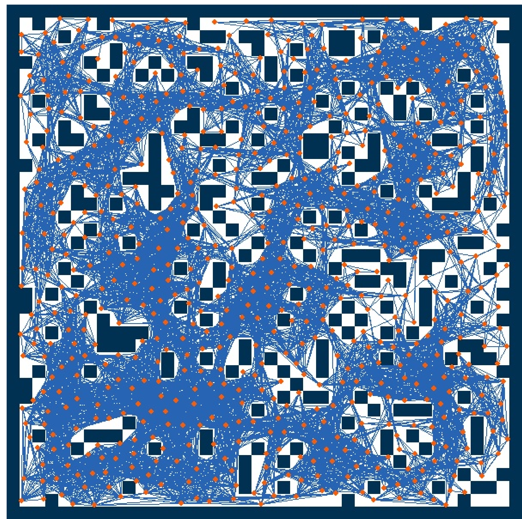
(b) -PRM Cluttered
