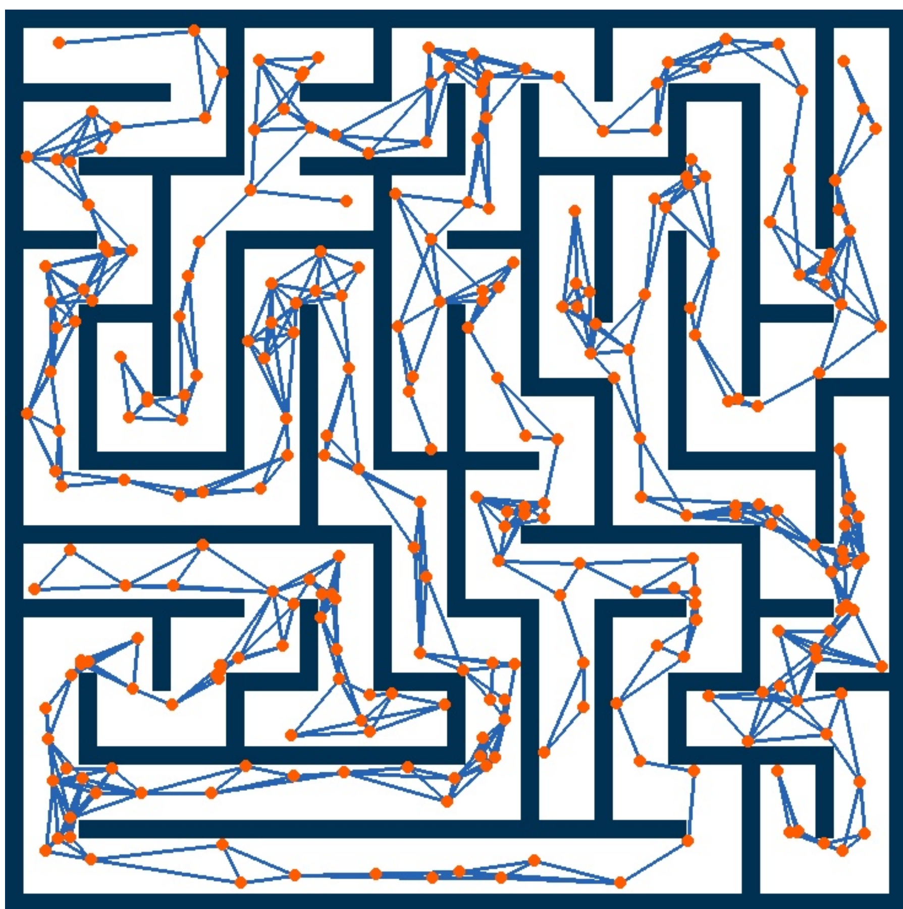
(c) SPARS2 Maze
