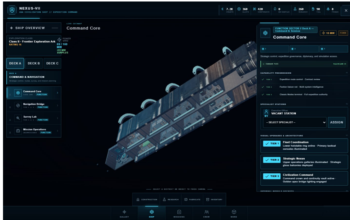
Landscape diagnostic overview
