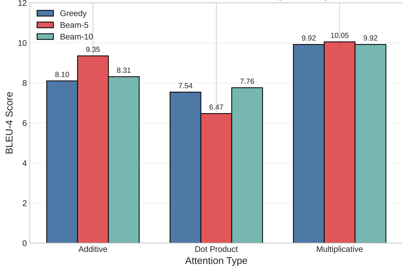
BLEU-4: Attention Mechanisms (TF=50%)
