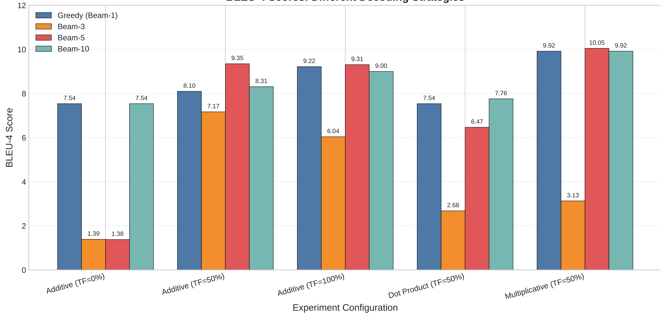
BLEU-4 Scores: Different Decoding Strategies
