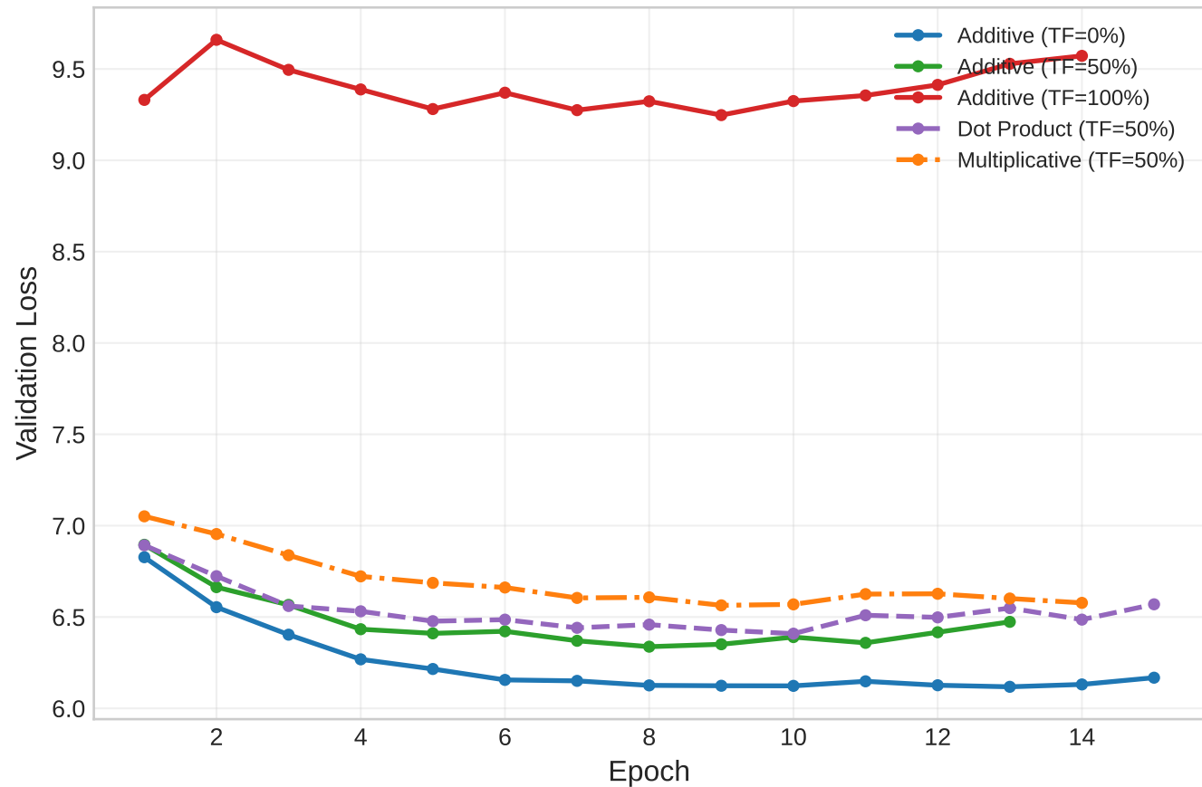
Validation Loss Curves
