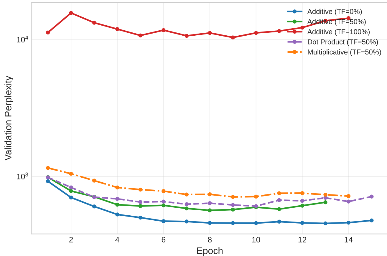
Validation Perplexity Curves
