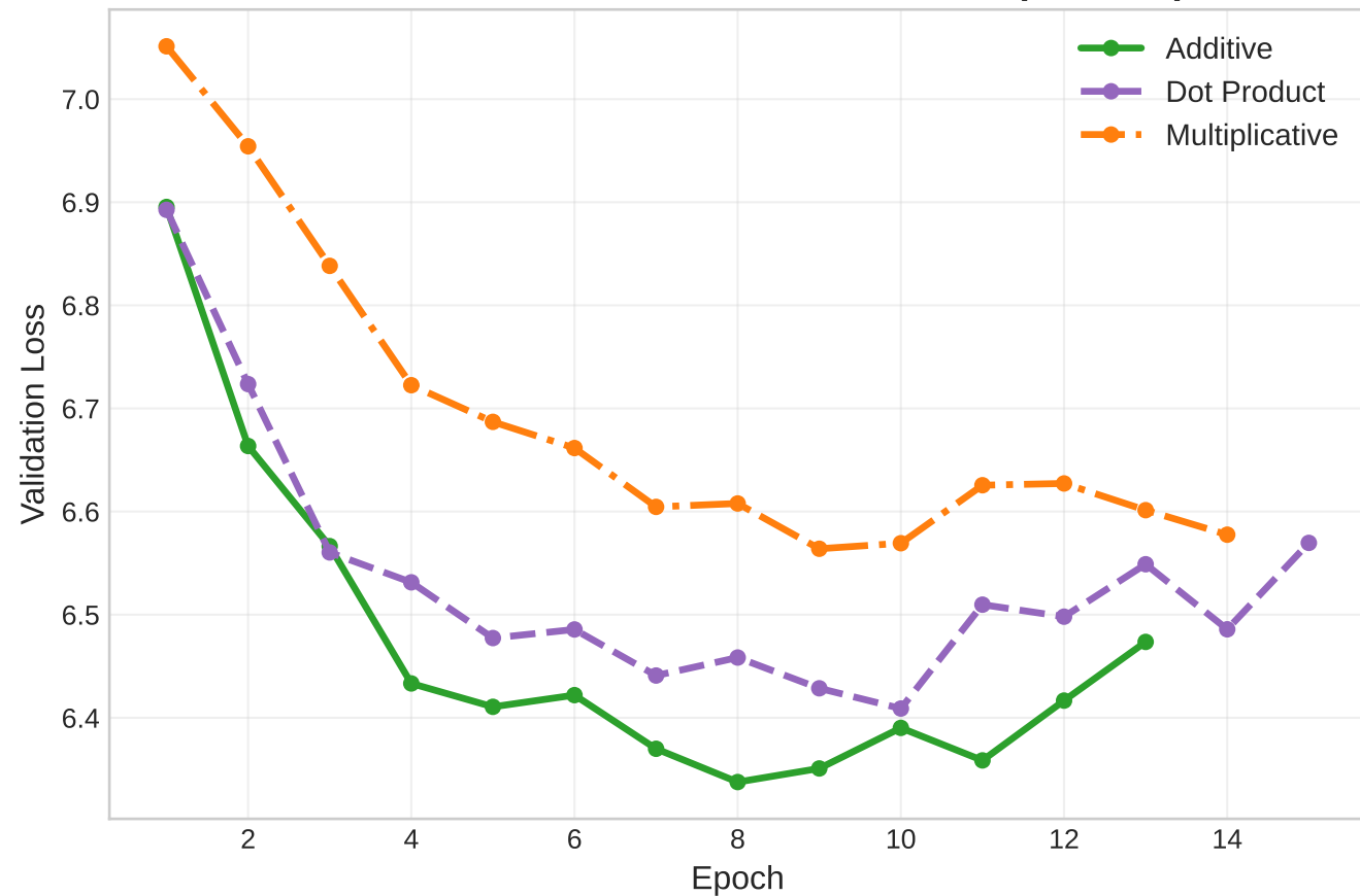
Validation Loss: Attention Mechanisms (TF=50%)
