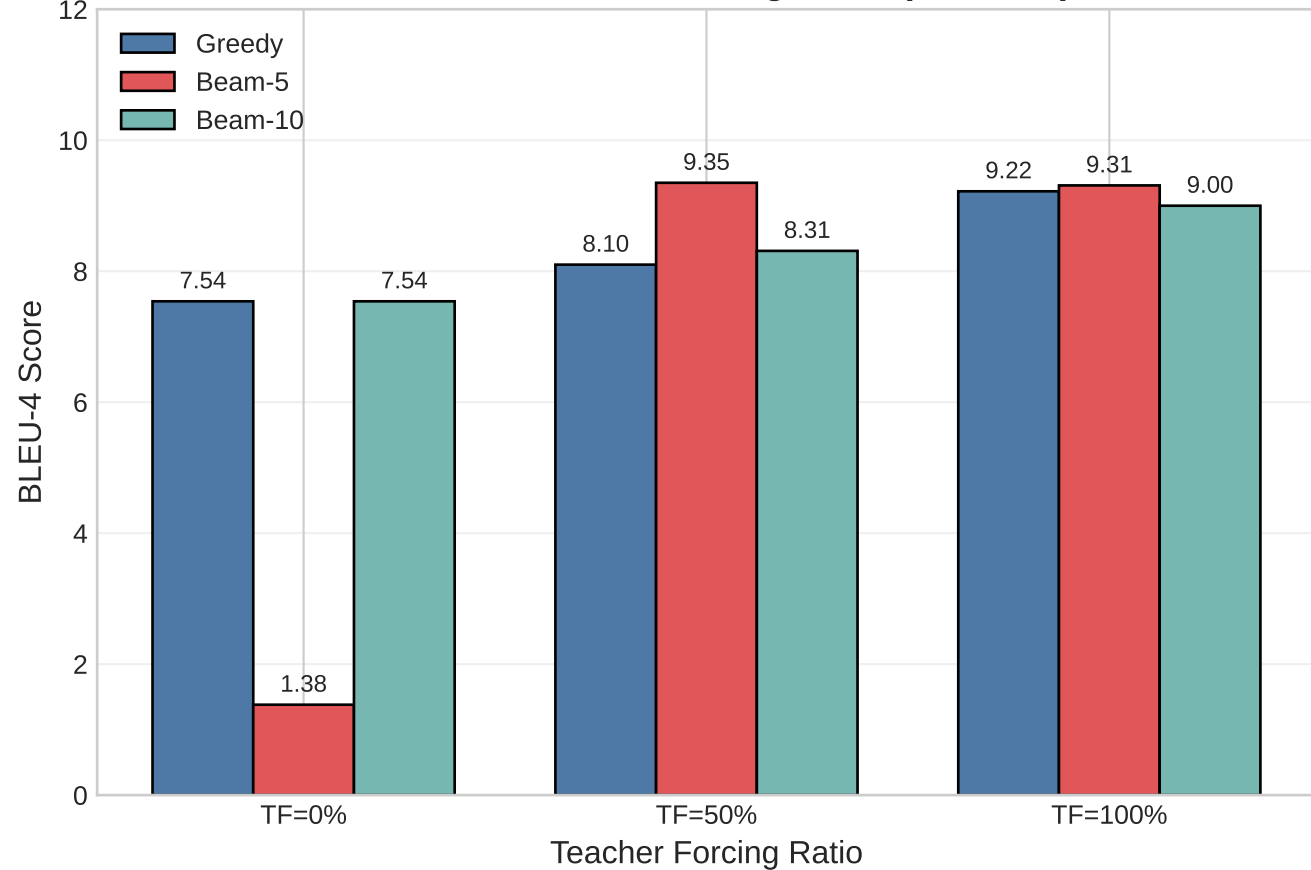
BLEU-4: Teacher Forcing Ratio (Additive)
