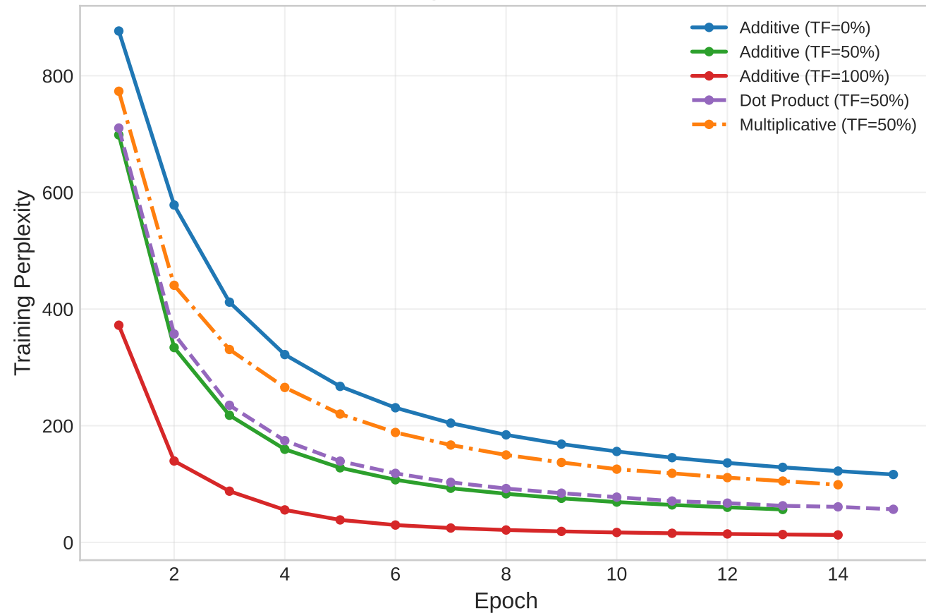
Training Perplexity Curves
