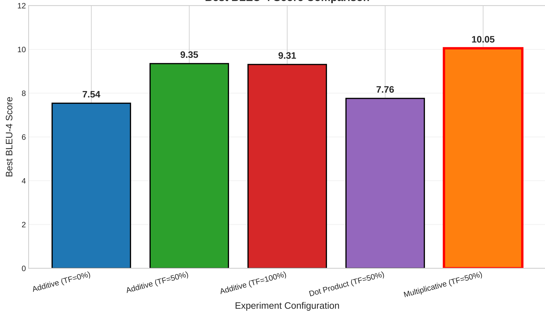
Best BLEU-4 Score Comparison
