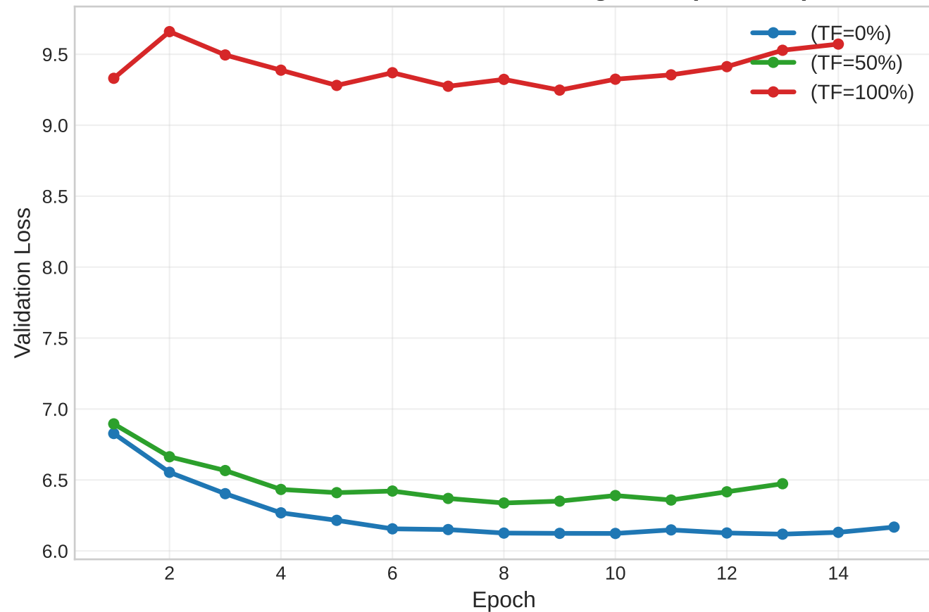
Validation Loss: Teacher Forcing Ratio (Additive)
