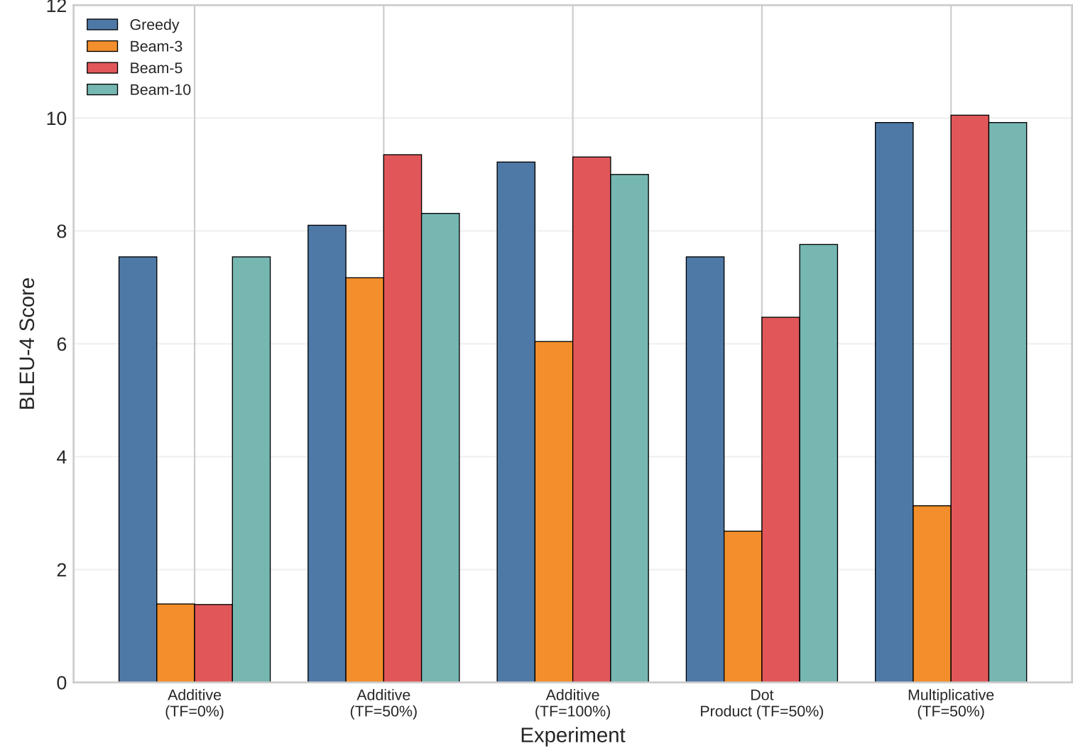
(c) BLEU-4 Scores by Decoding Strategy
