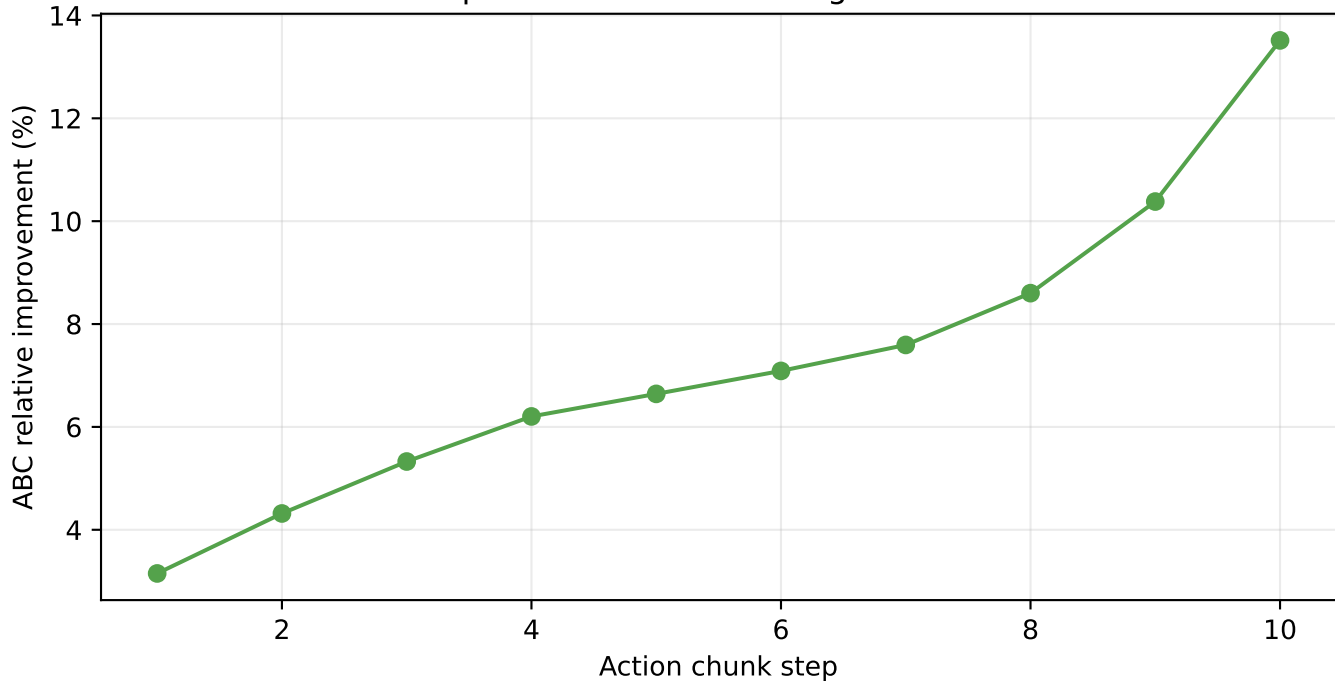
ABC Improvement Grows Along Chunk Horizon
