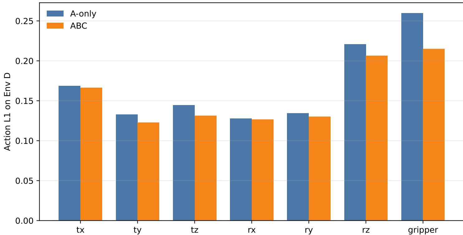
Zero-shot Action Error by Dimension
