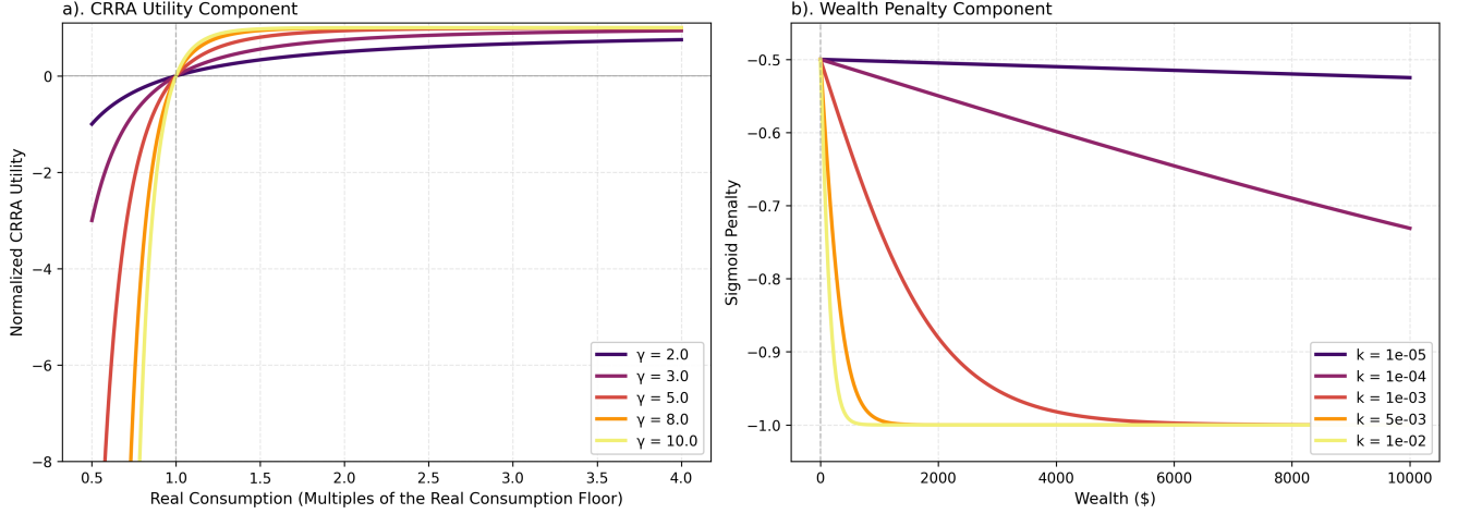
Figure 6: Components of the cost function used in optimization. Panel (a) shows normalized CRRA utility \tilde{U}_\gamma(x) as a function of normalized consumption x = c/\underline{c} for different risk aversion coefficients ( \gamma = 2, 3, 5, 8, 10 ). Higher \gamma values produce steeper, more concave utility curves reflecting greater risk aversion. Panel (b) shows the sigmoid wealth penalty -\sigma(kw) for different steepness parameters ( k = 10^{-5} to 10^{-2} ). Larger k values create sharper “knees” that more aggressively penalize low and negative wealth outcomes.
