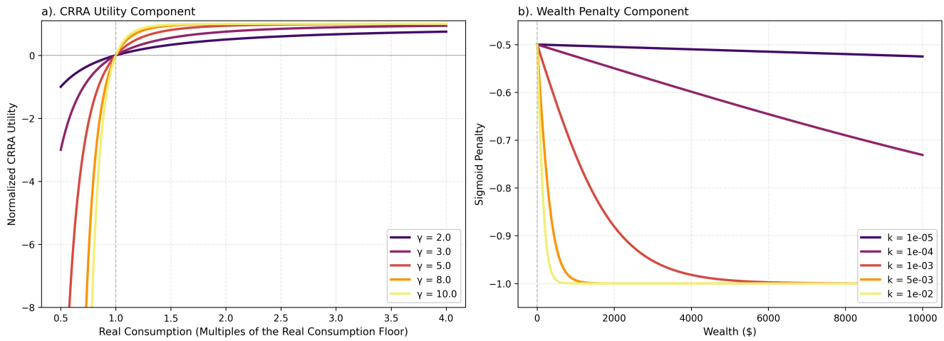
Figure 6: Components of the cost function used in optimization. Panel (a) shows normalized CRRA utility \tilde{U}_\gamma(x) as a function of normalized consumption x = c/\underline{c} for different risk aversion coefficients ( \gamma = 2, 3, 5, 8, 10 ). Higher \gamma values produce steeper, more concave utility curves reflecting greater risk aversion. Panel (b) shows the sigmoid wealth penalty -\sigma(kw) for different steepness parameters ( k = 10^{-5} to 10^{-2} ). Larger k values create sharper “knees” that more aggressively penalize low and negative wealth outcomes.
