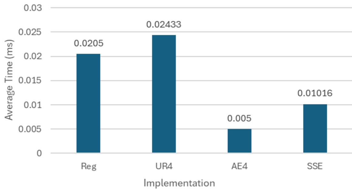
Average Dot Product time size=32768
