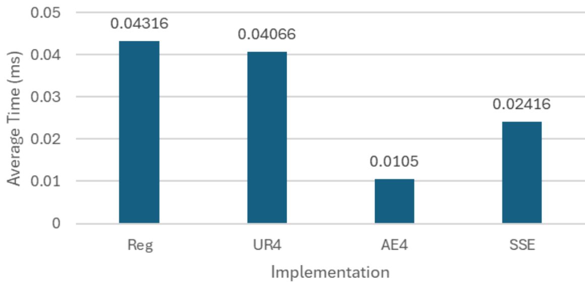
Average Dot Product time size=65536
