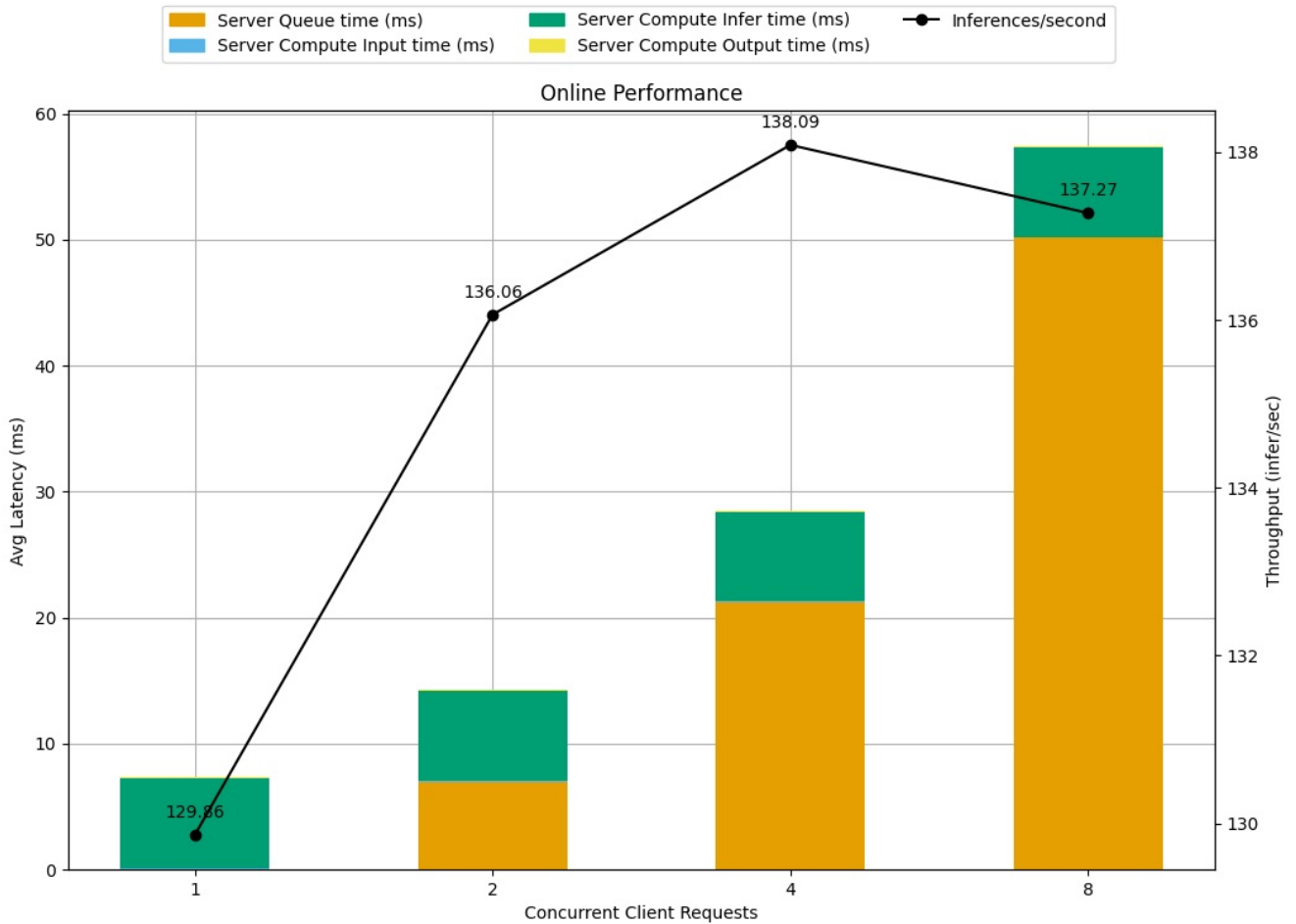
Latency Breakdown for Online Performance of selfie_segmentation_config_0
