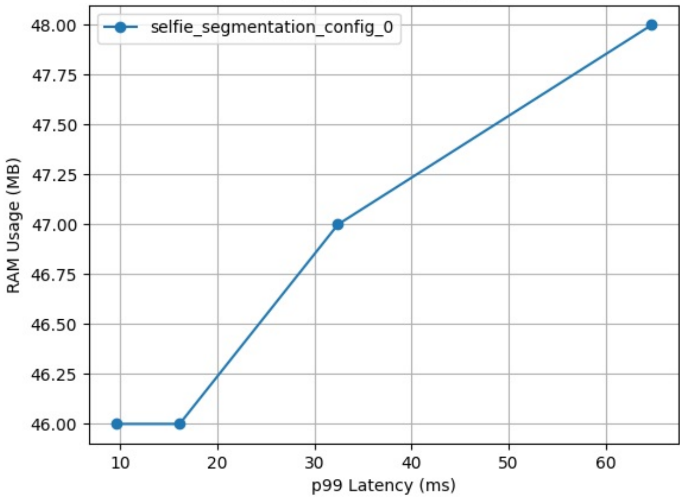
RAM Usage vs. Latency
