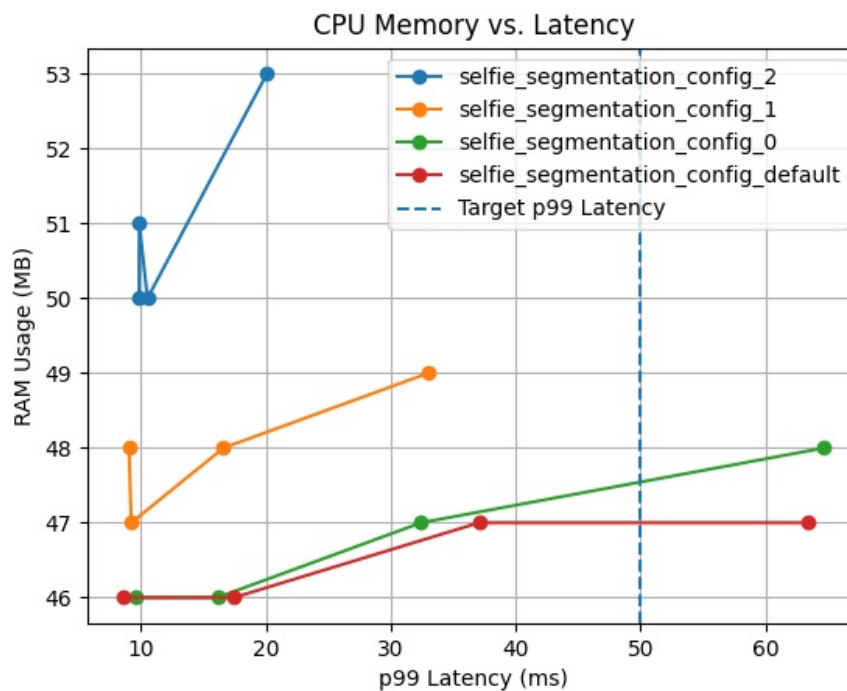
CPU Memory vs. Latency curves for 3 best configurations.
