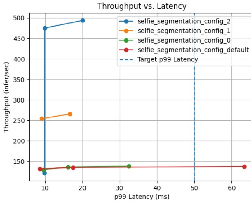
Throughput vs. Latency curves for 3 best configurations.
