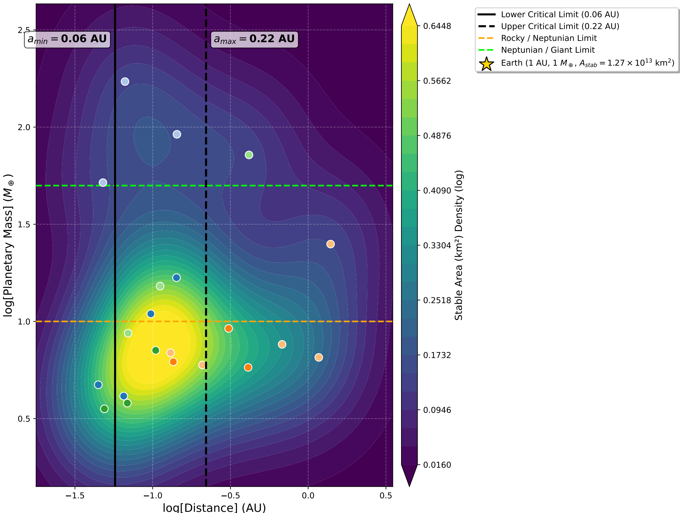
Systems with 3 planets
