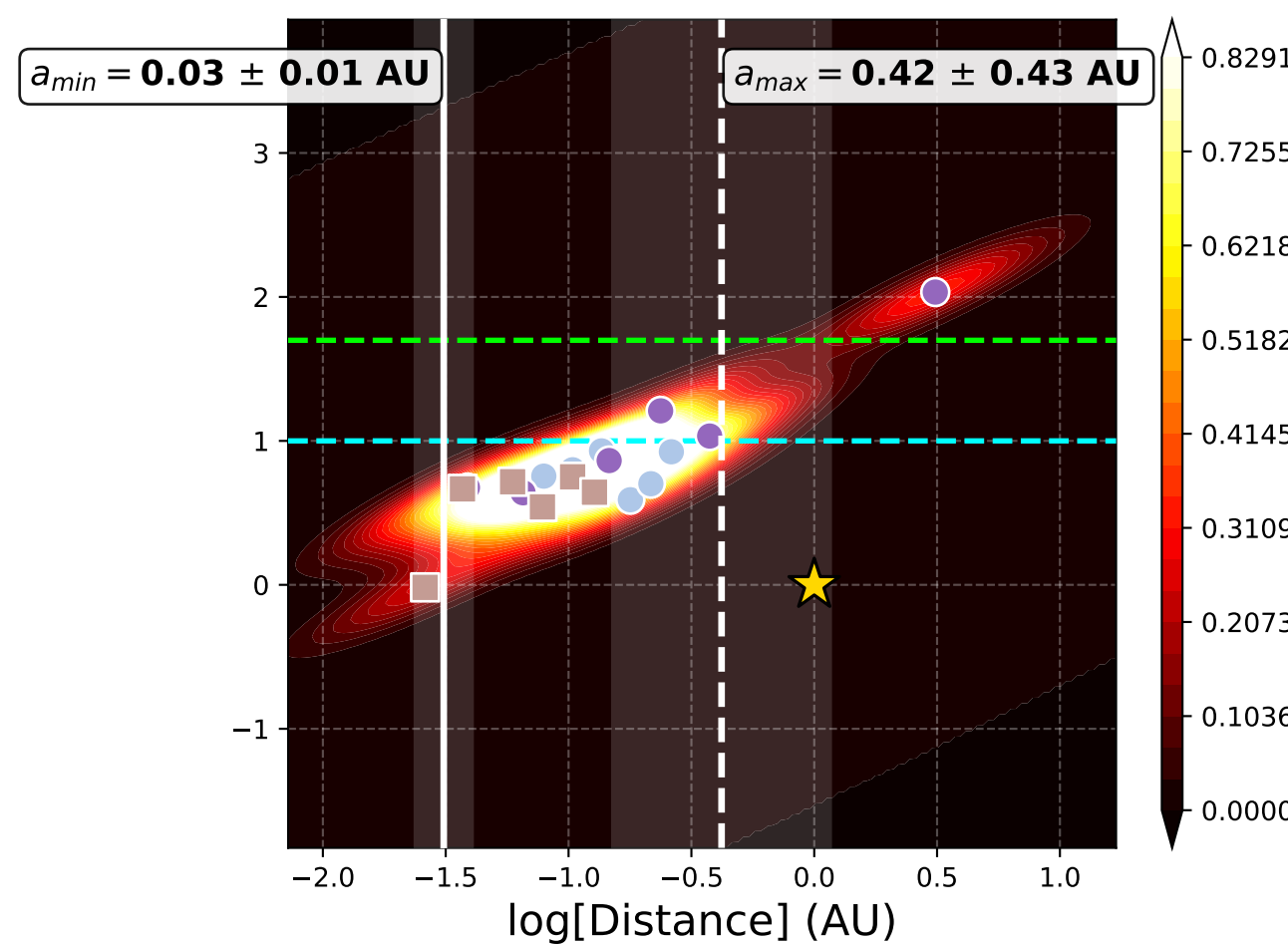
Systems with 6 planets
