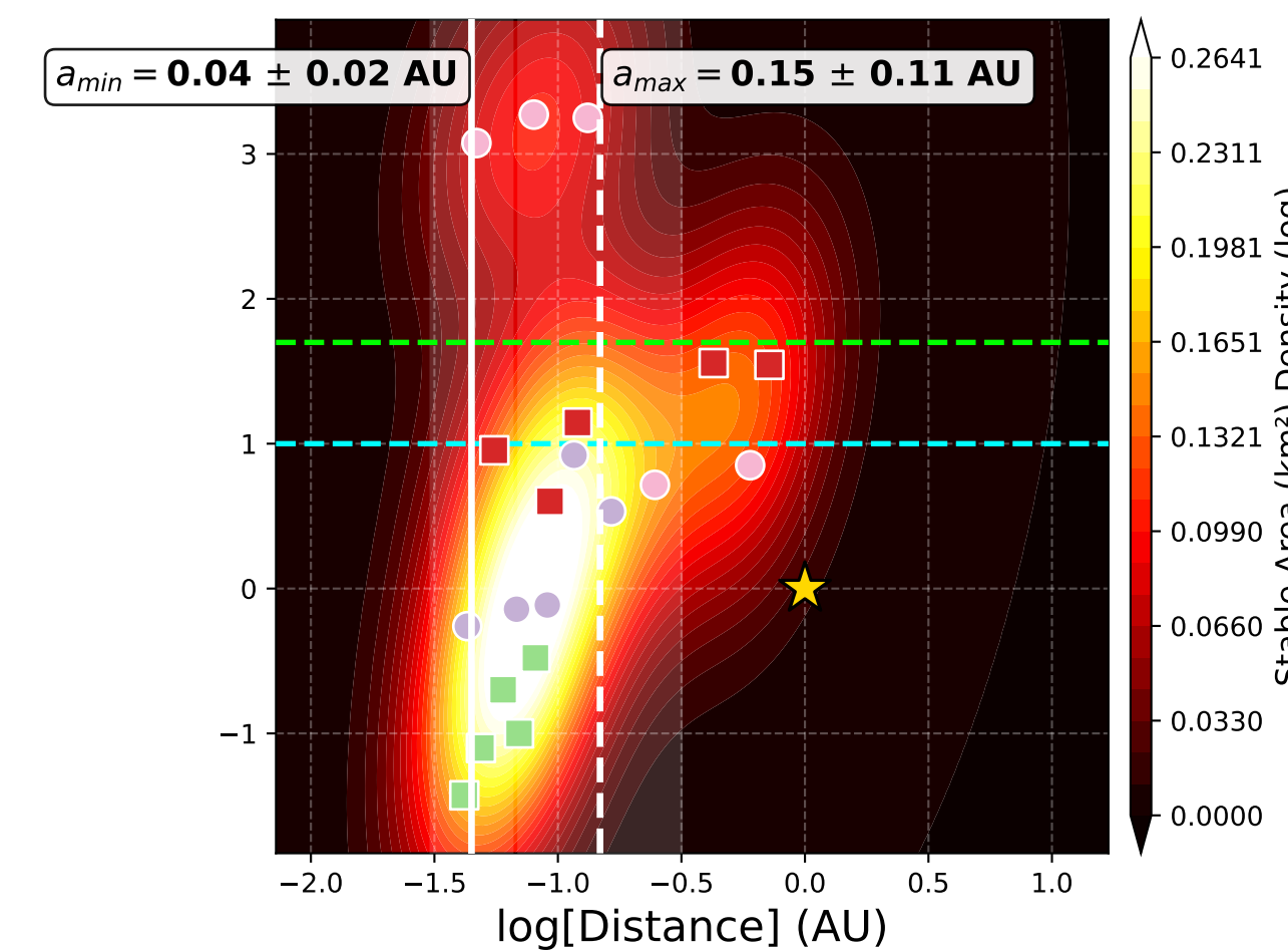
Systems with 5 planets
