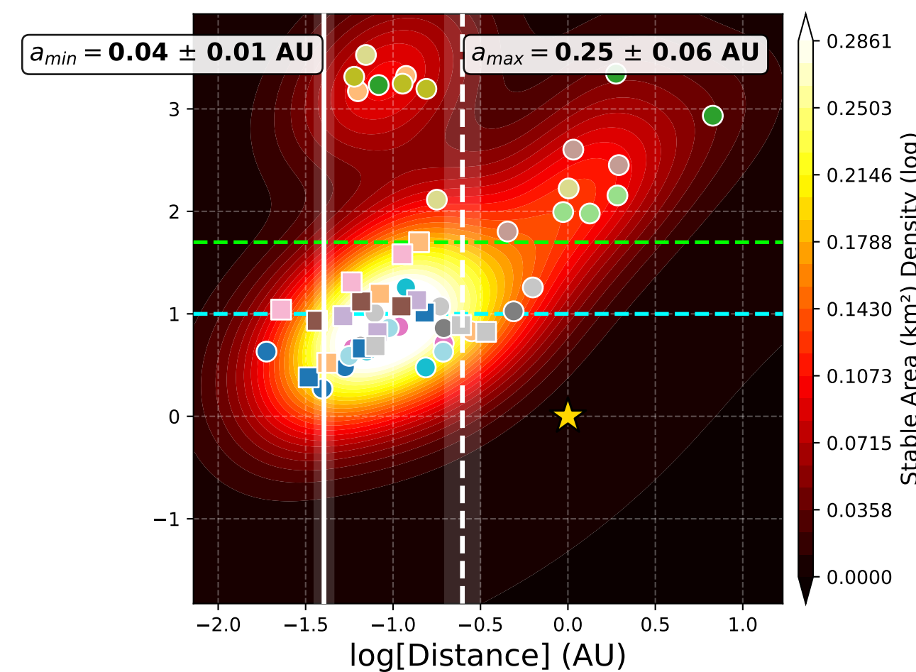
Systems with 3 planets
