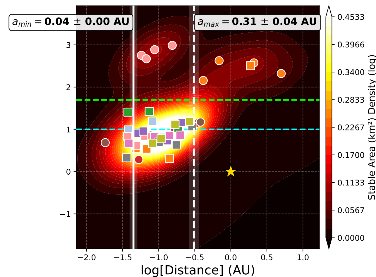
Systems with 4 planets
