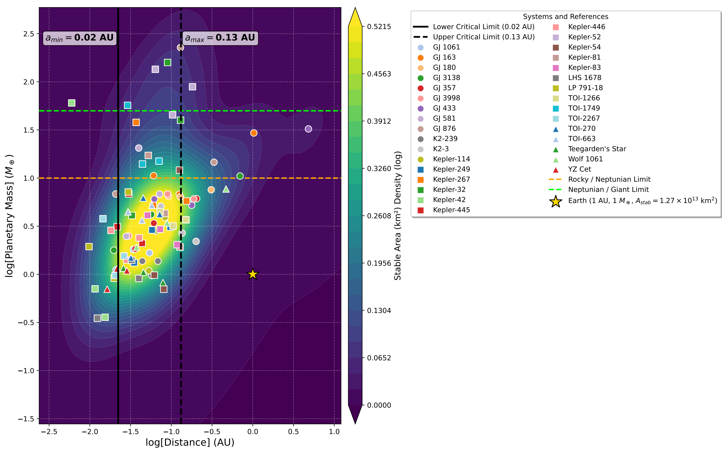
Systems with 4 planets
