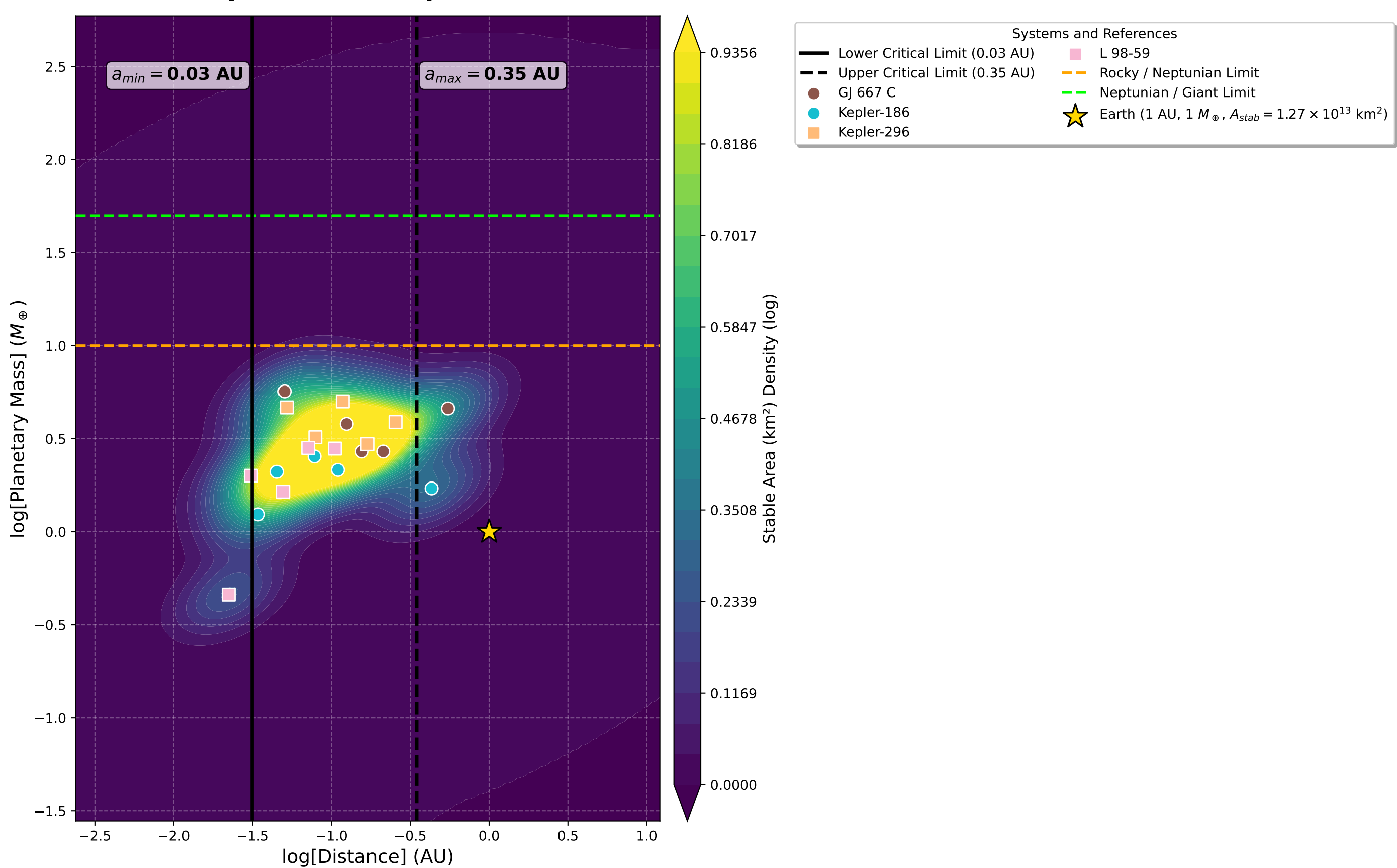
Systems with 7 planets
