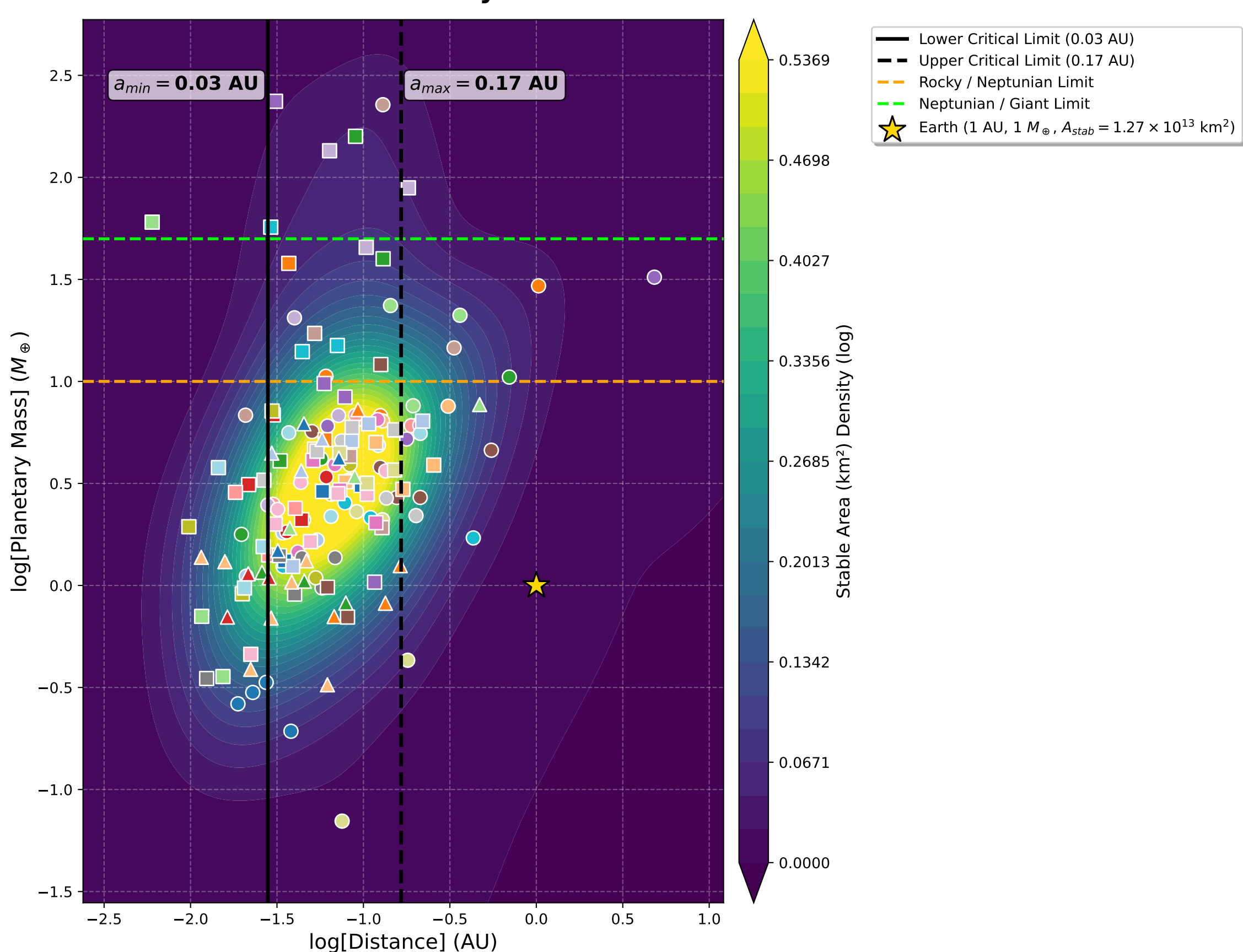
Systems with 3 planets
