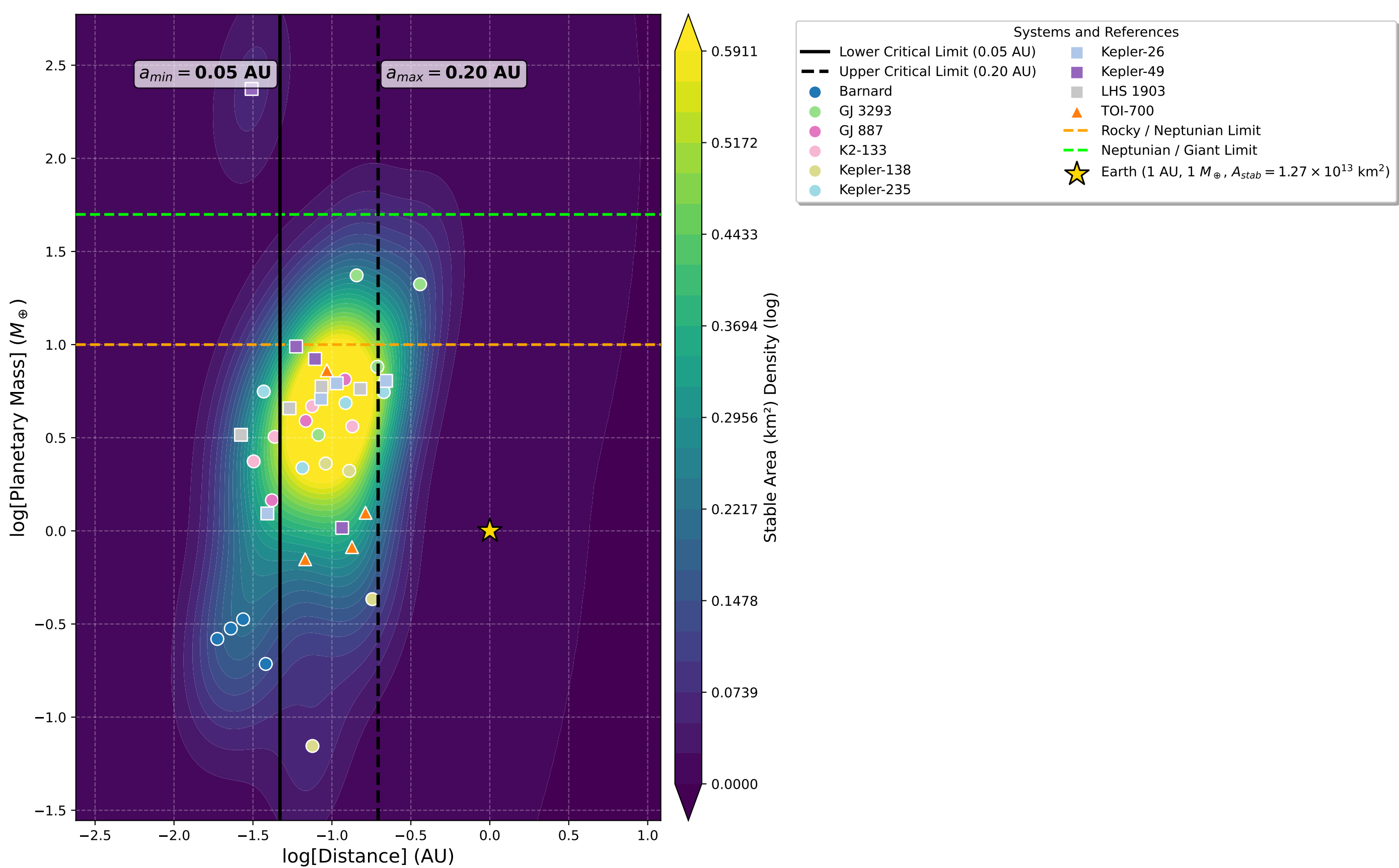
Systems with 5 planets
