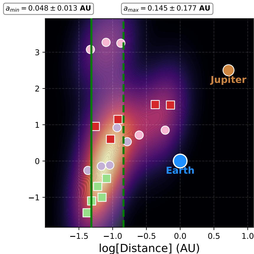
Systems with 5 planets
