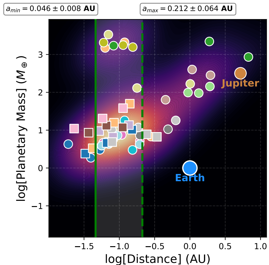
Systems with 3 planets
