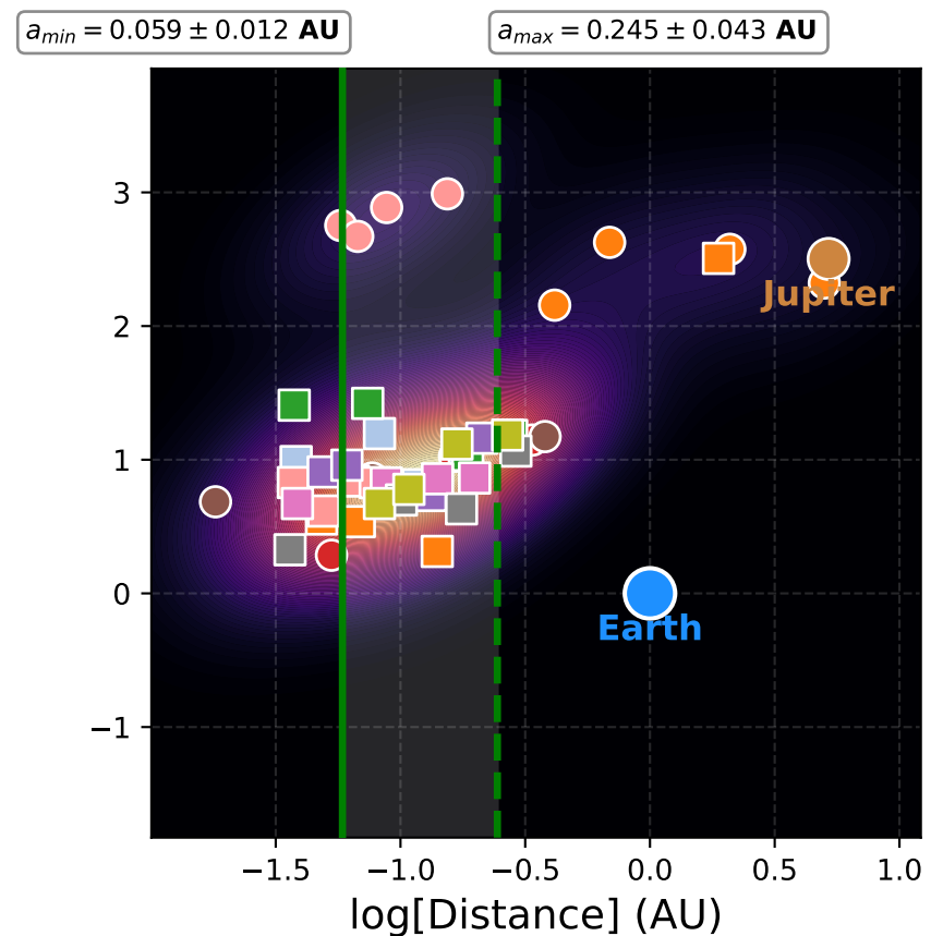
Systems with 4 planets
