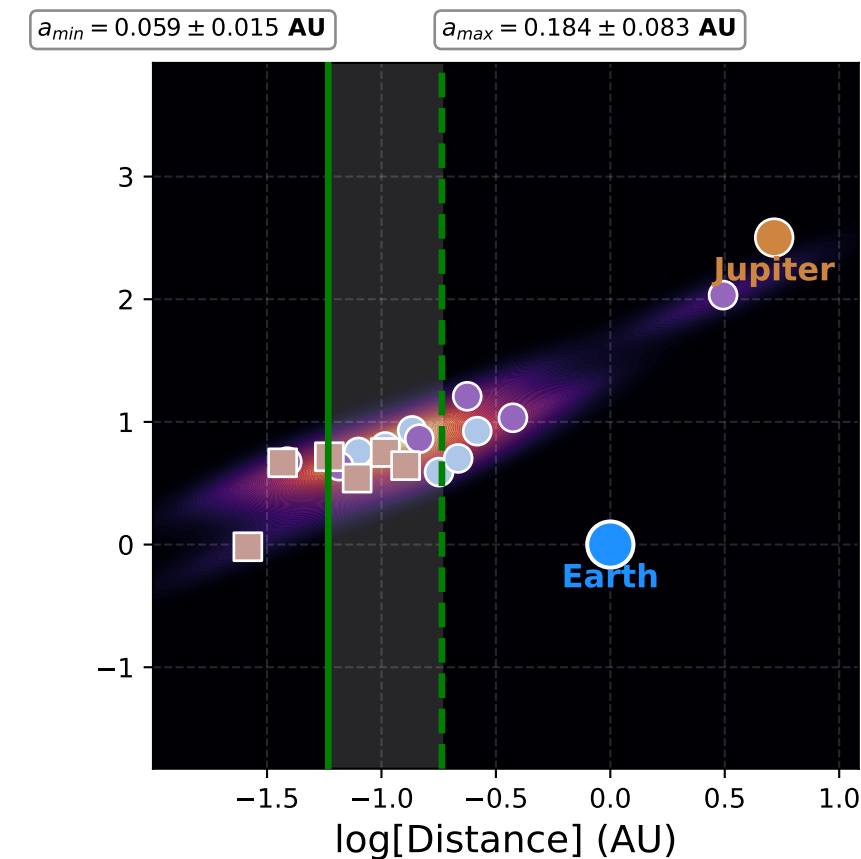
Systems with 6 planets
