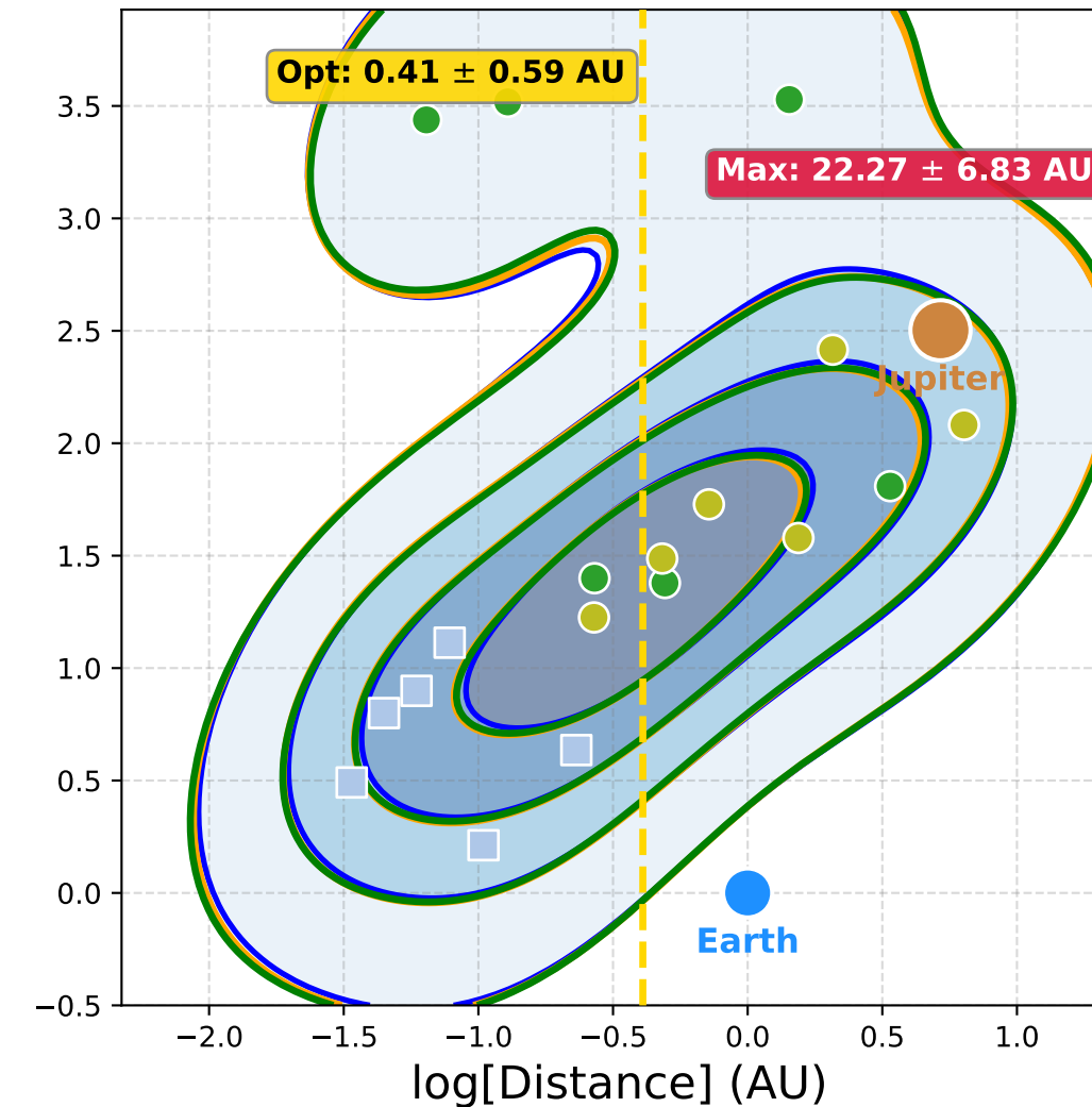
6-Planet Systems (N=3 systems)
