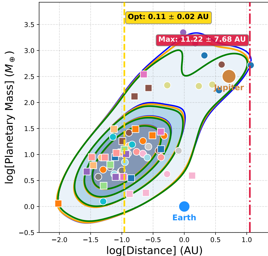
3-Planet Systems (N=21 systems)
