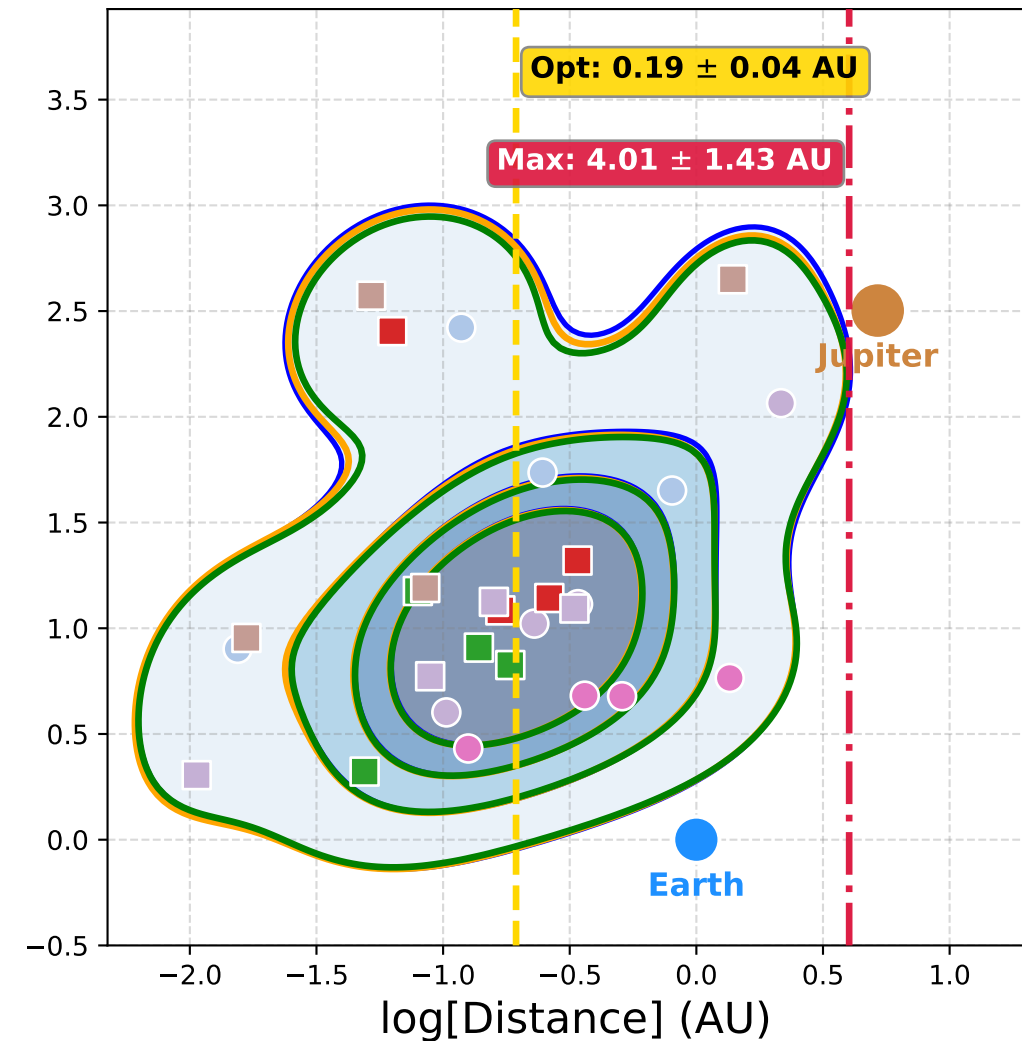
4-Planet Systems (N=7 systems)
