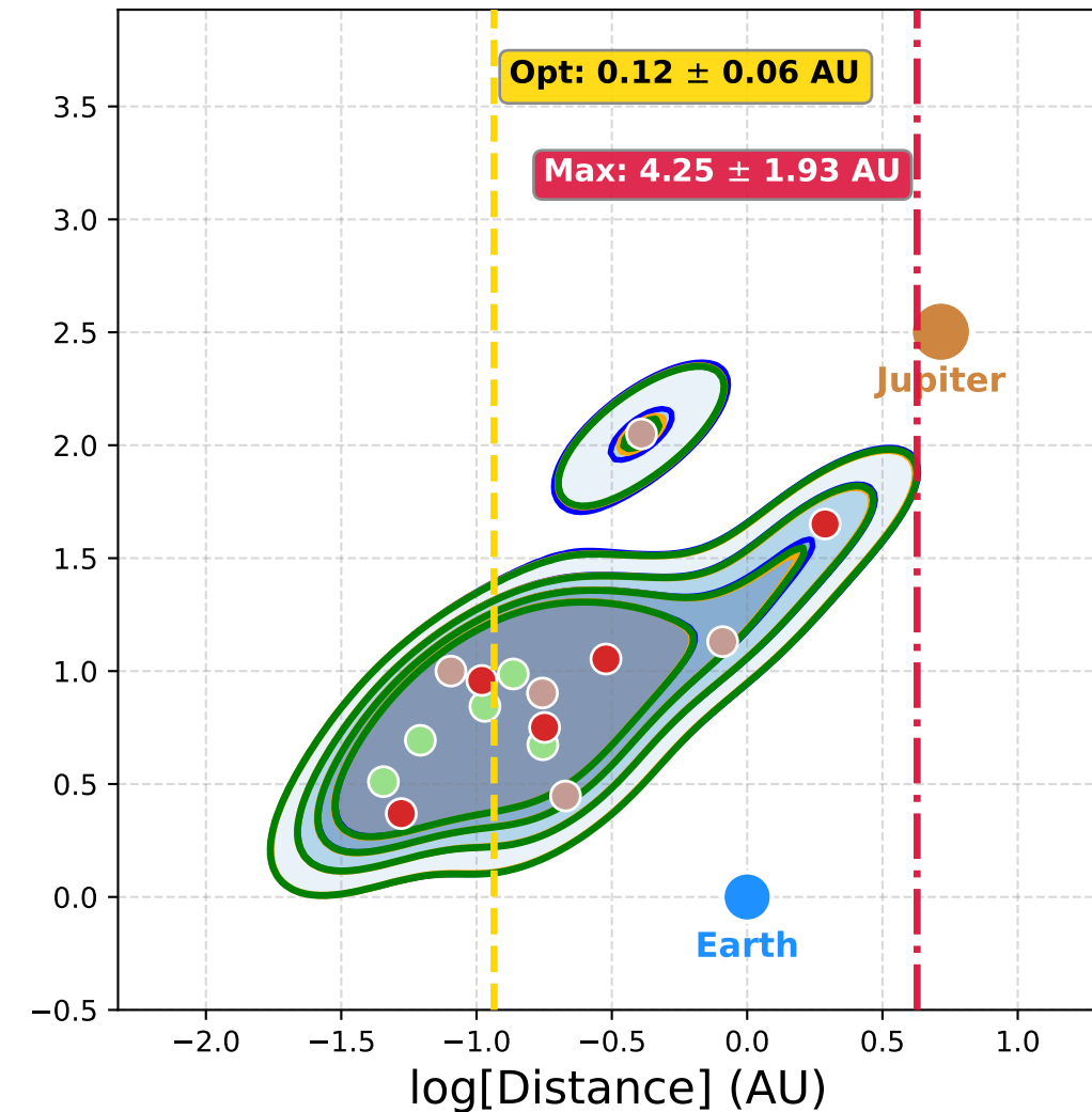
5-Planet Systems (N=3 systems)
