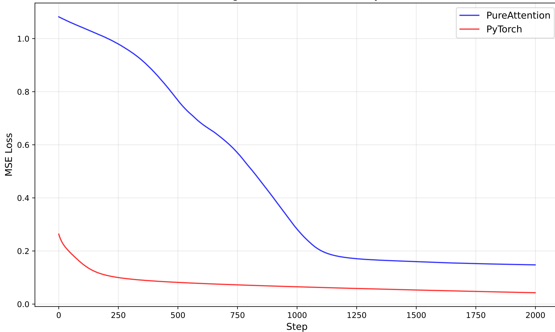
Denoising Task: PureAttention vs PyTorch
