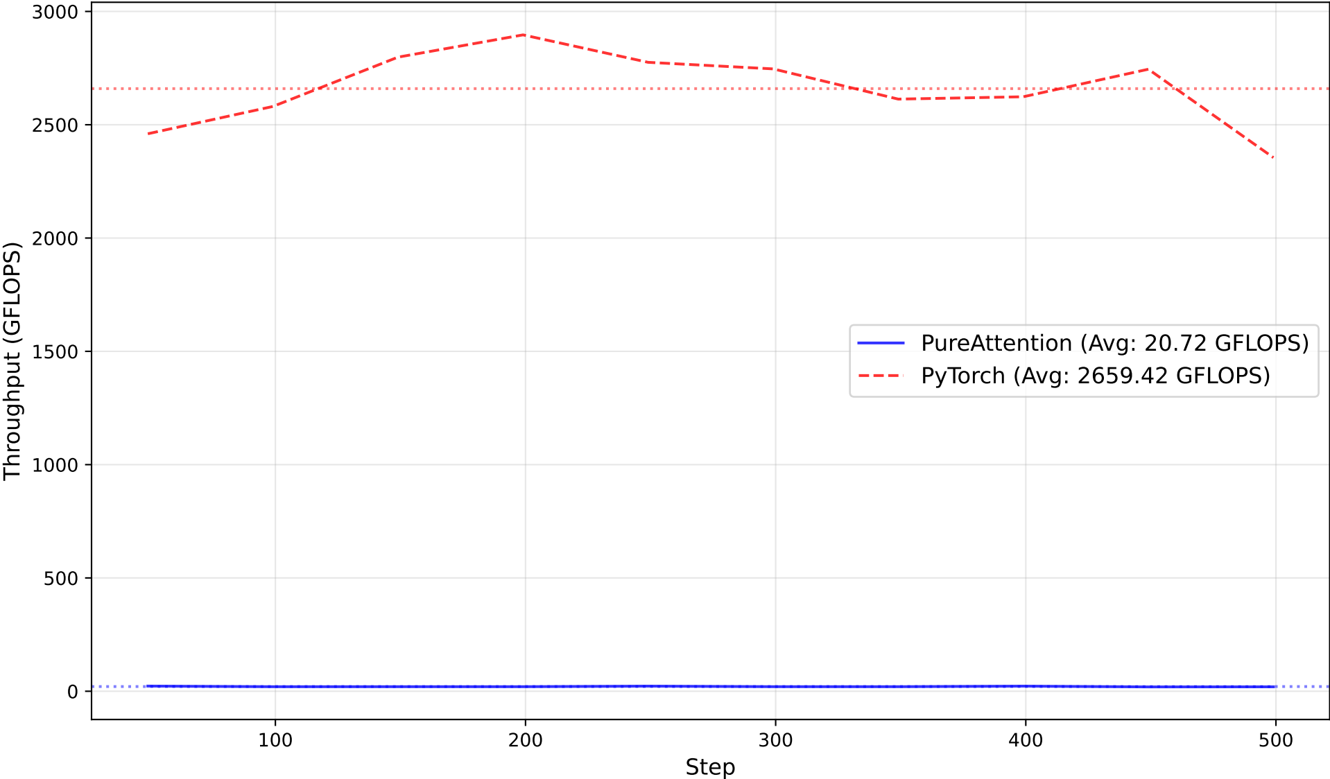
Performance Benchmark: GFLOPS Comparison
