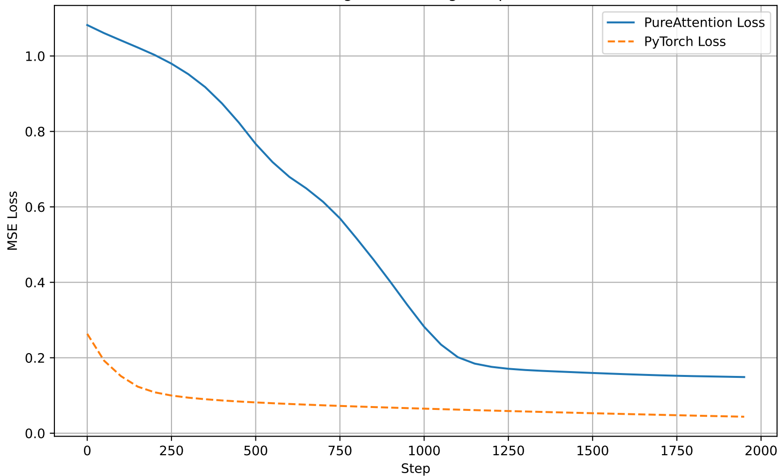
Denoising Task Training Comparison
