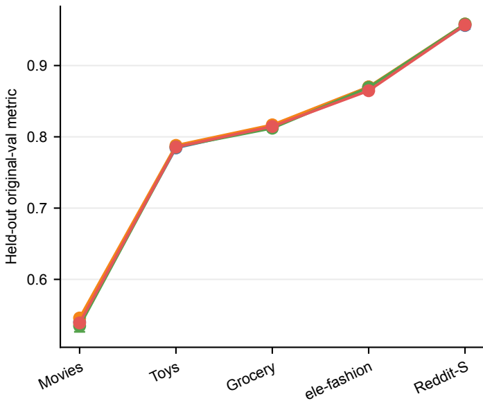
Accuracy
