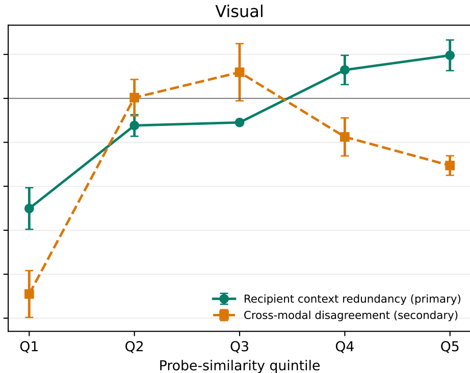
Toys: context-conditioned utility (mean \pm seed SD)
