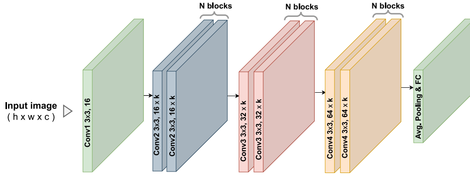
Fig. 4. Our WRN base model architecture implemented in the benchmark. The blocks of the architecture are explained in Fig. 5.
