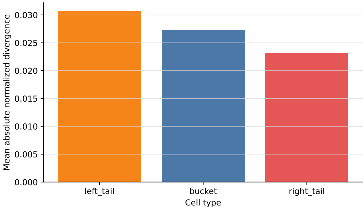
Cell-Level Wedge by Bucket Type
