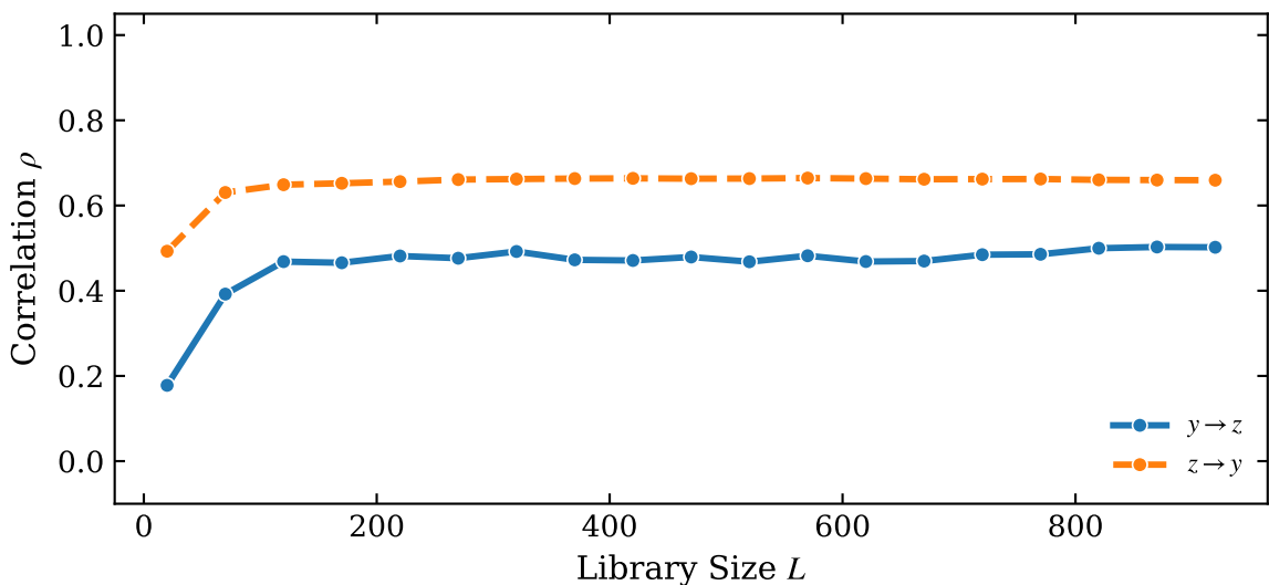
E=4, \tau=8 (with ds)
