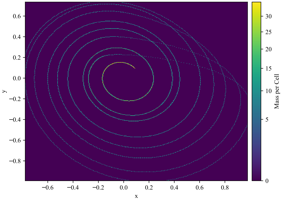
Rössler invariant measure (x-y projection)
