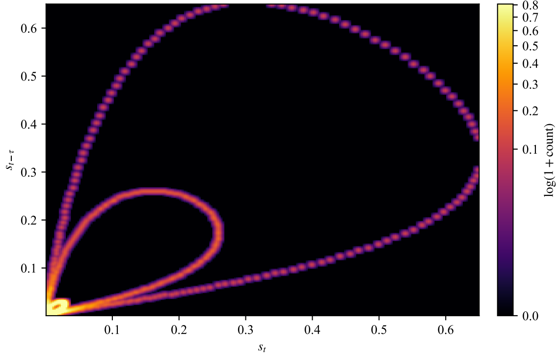
z delay-invariant measure, \tau = 30
