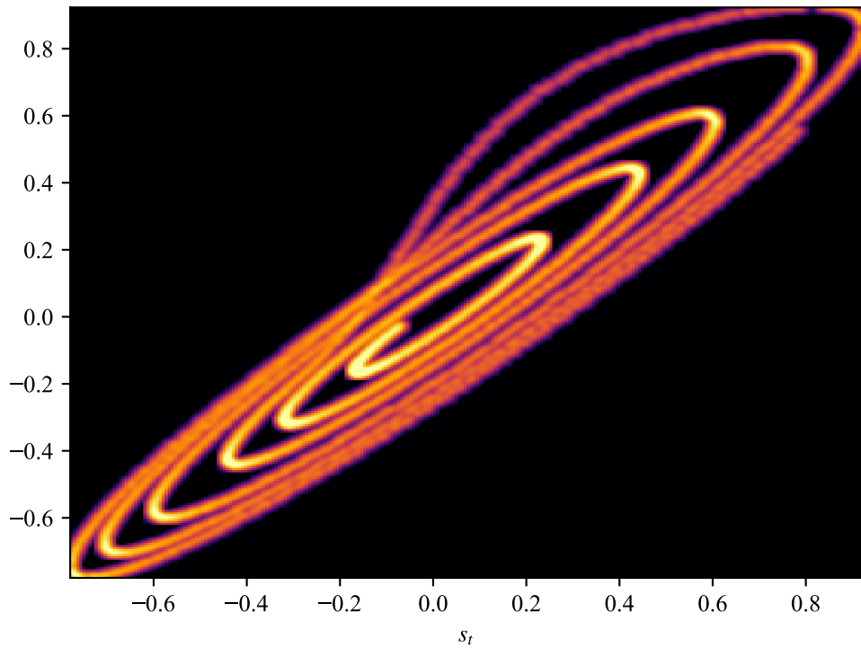
x delay-invariant measure, \tau = 30
