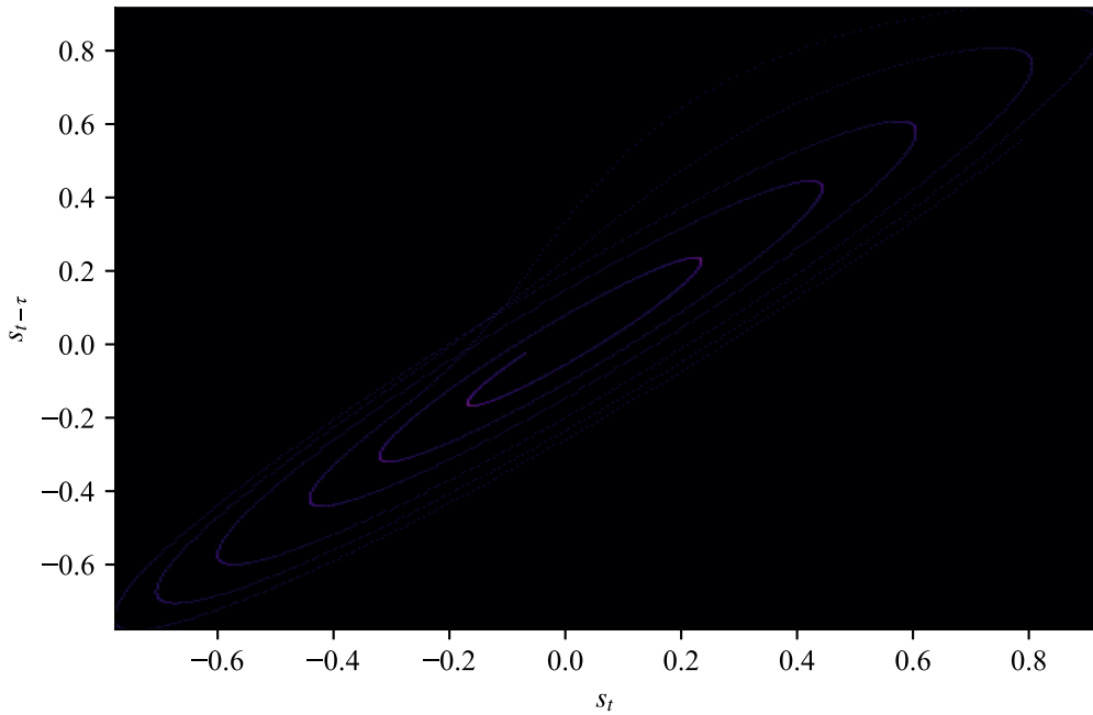
x delay-invariant measure, \tau = 30
