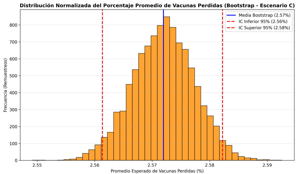
Figura 5.22: histograma Bootstrap
