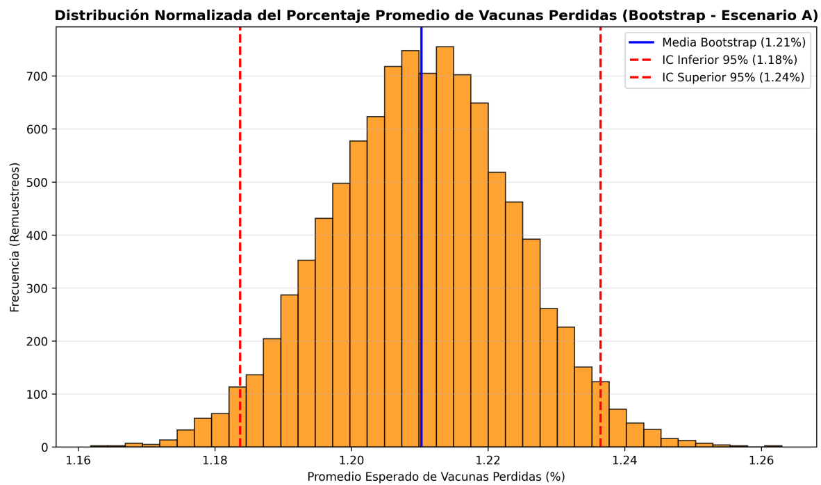
Figura 5.20: histograma Bootstrap
