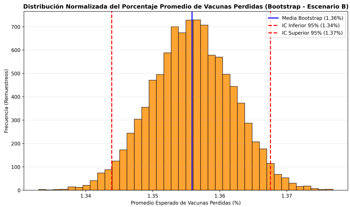
Figura 5.21: histograma Bootstrap
