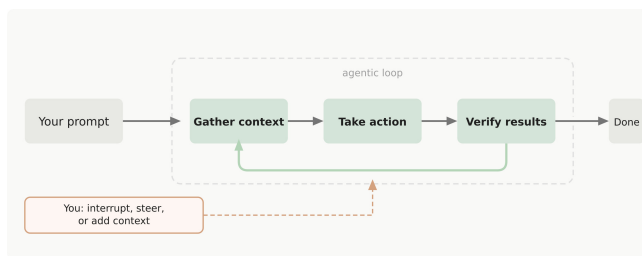
Figure 3: Claude Code's prompt processing architecture [4]
