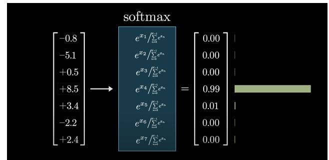
Figure 5: How the scalar values are turned into a probability distribution [21]
