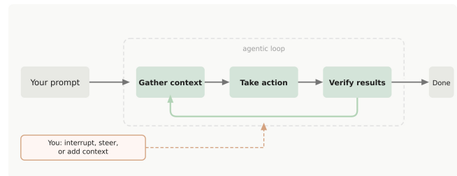
Figure 1: Claude Code's prompt processing architecture [4]
