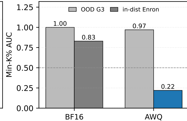
(b) MIA AUC, two non-member sets
