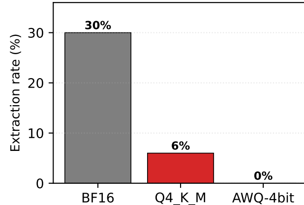
(a) Verbatim extraction (seed 42)
