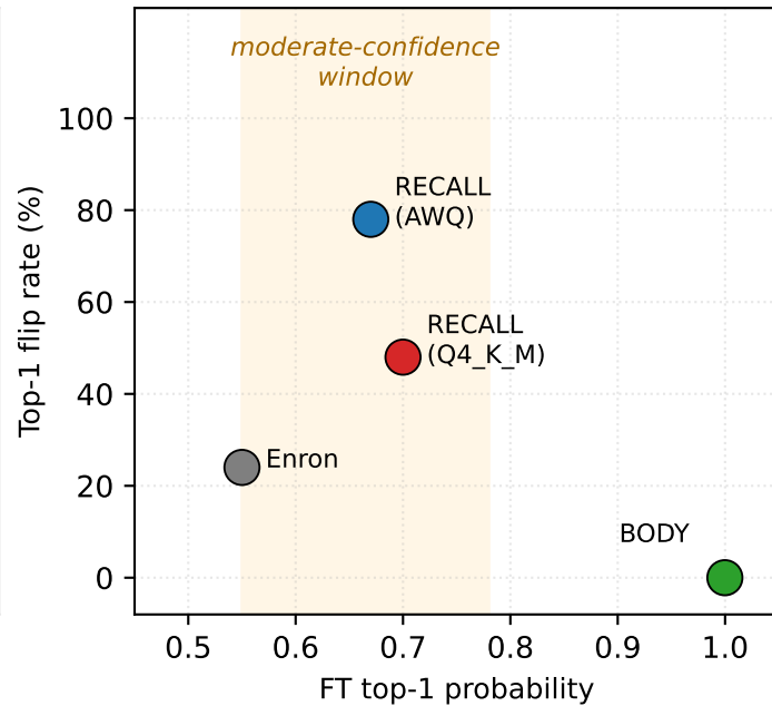
Factor 2: confidence window
