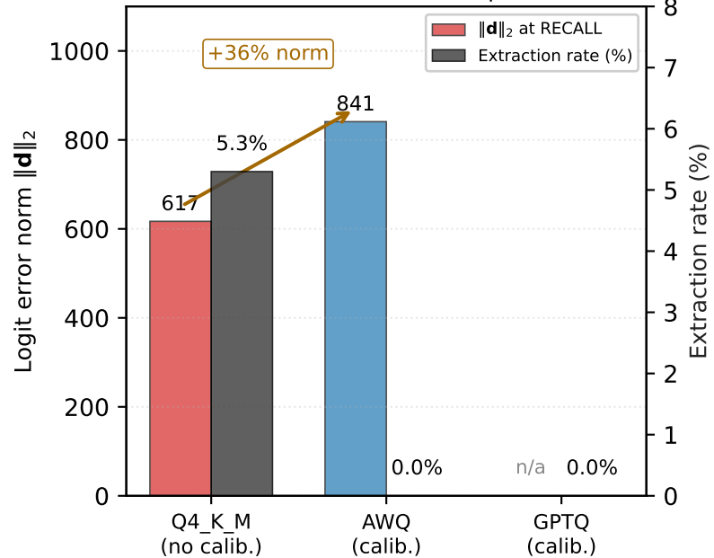
Factor 3: calibration amplifies
