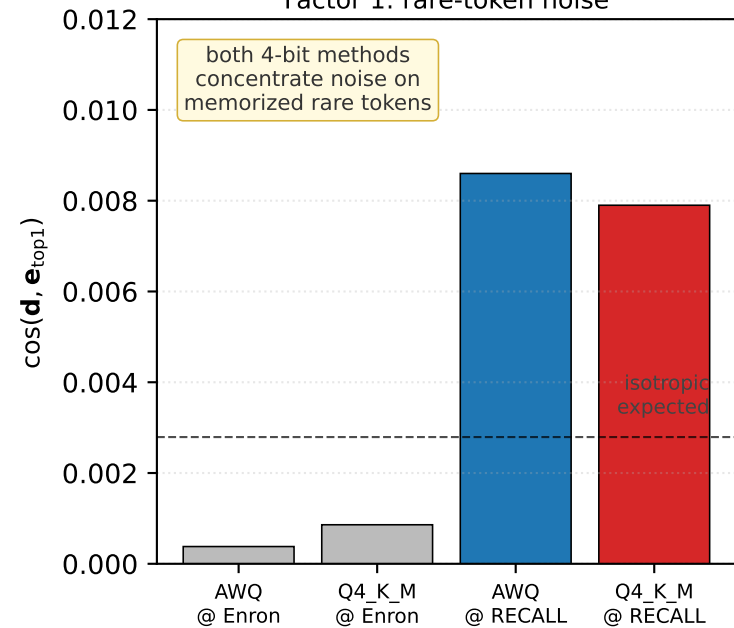
Factor 1: rare-token noise
