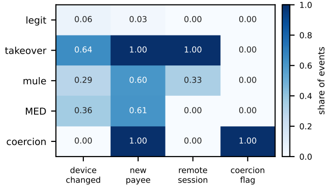
(c) signal presence per scenario
