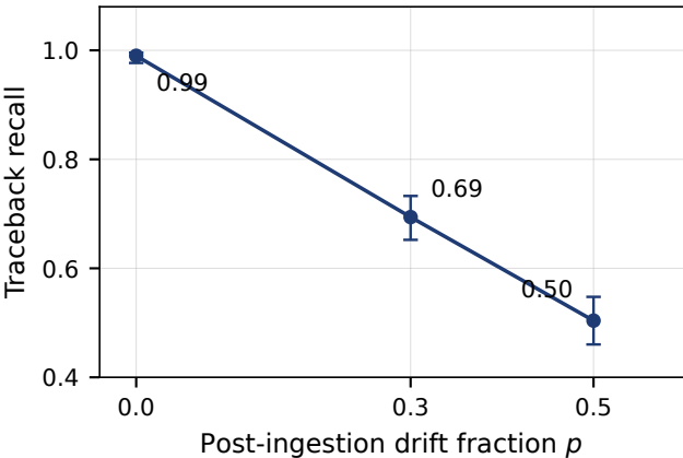
(a) Traceback recall vs. drift
