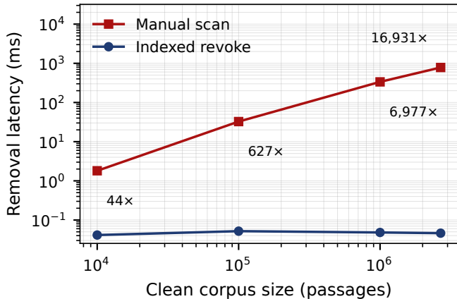
(b) Revocation latency vs. scale
