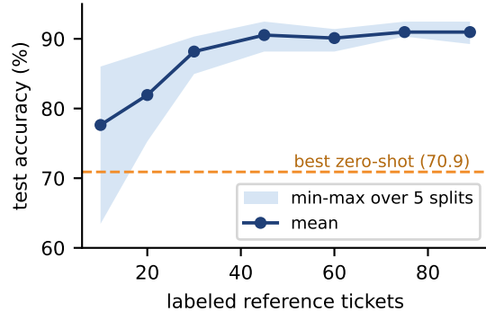
(b) accuracy vs. reference-set size
